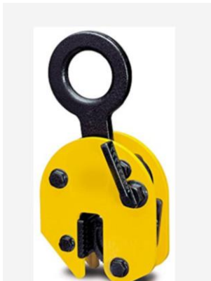
Line 15: Supply 1-ton heavy duty vertical plate grabber
