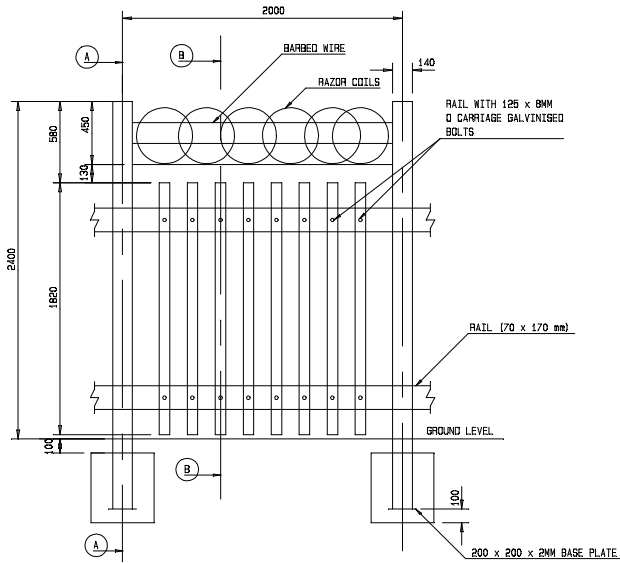
FRONT VIEW OF CONCRETE PALISADE SECTION
