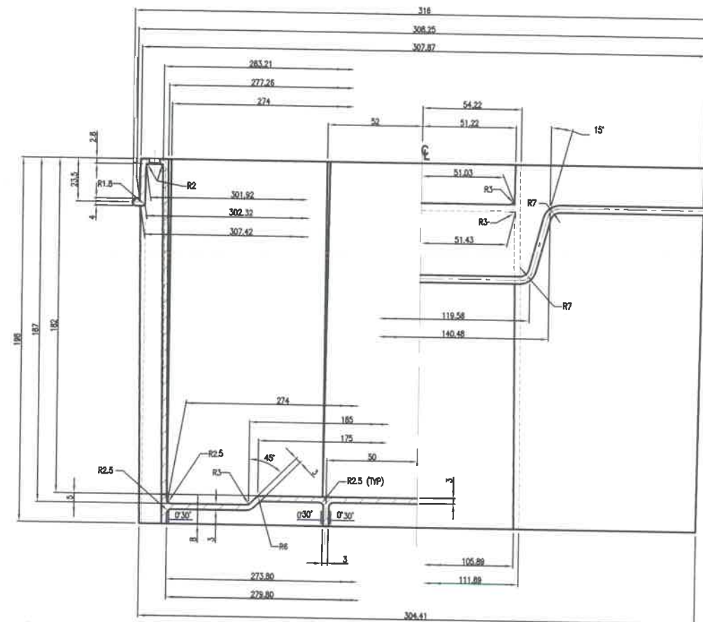
SECTION B-B
