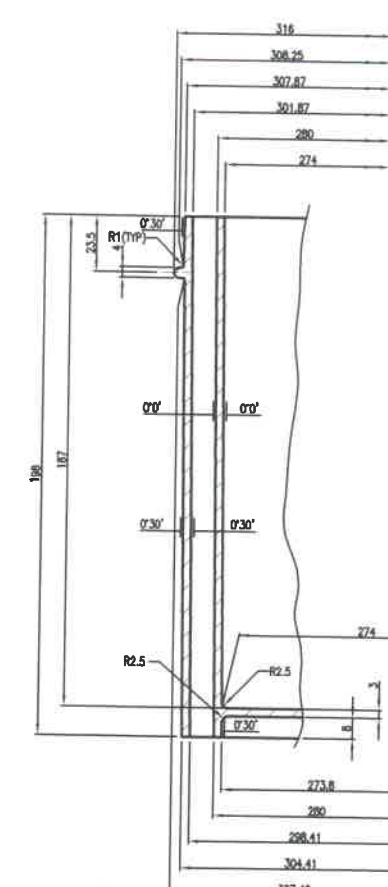
SCRAP SECTION D-D
