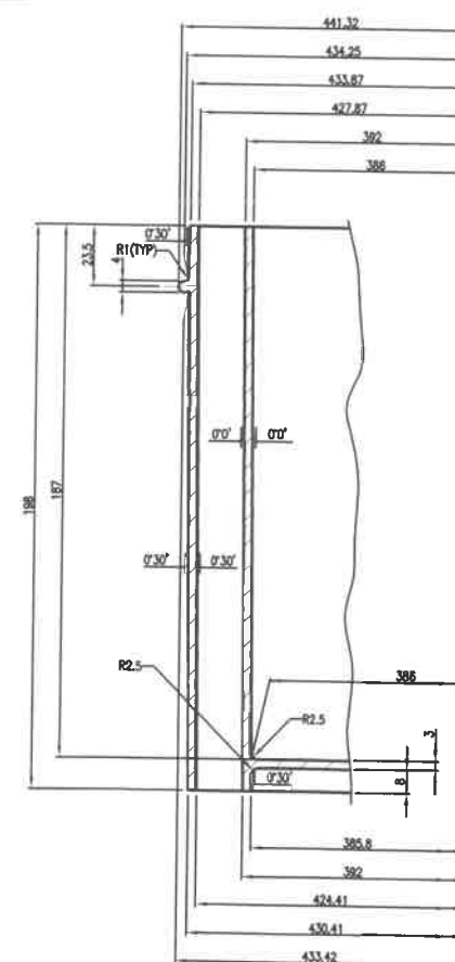
SCRAP SECTION C-C
