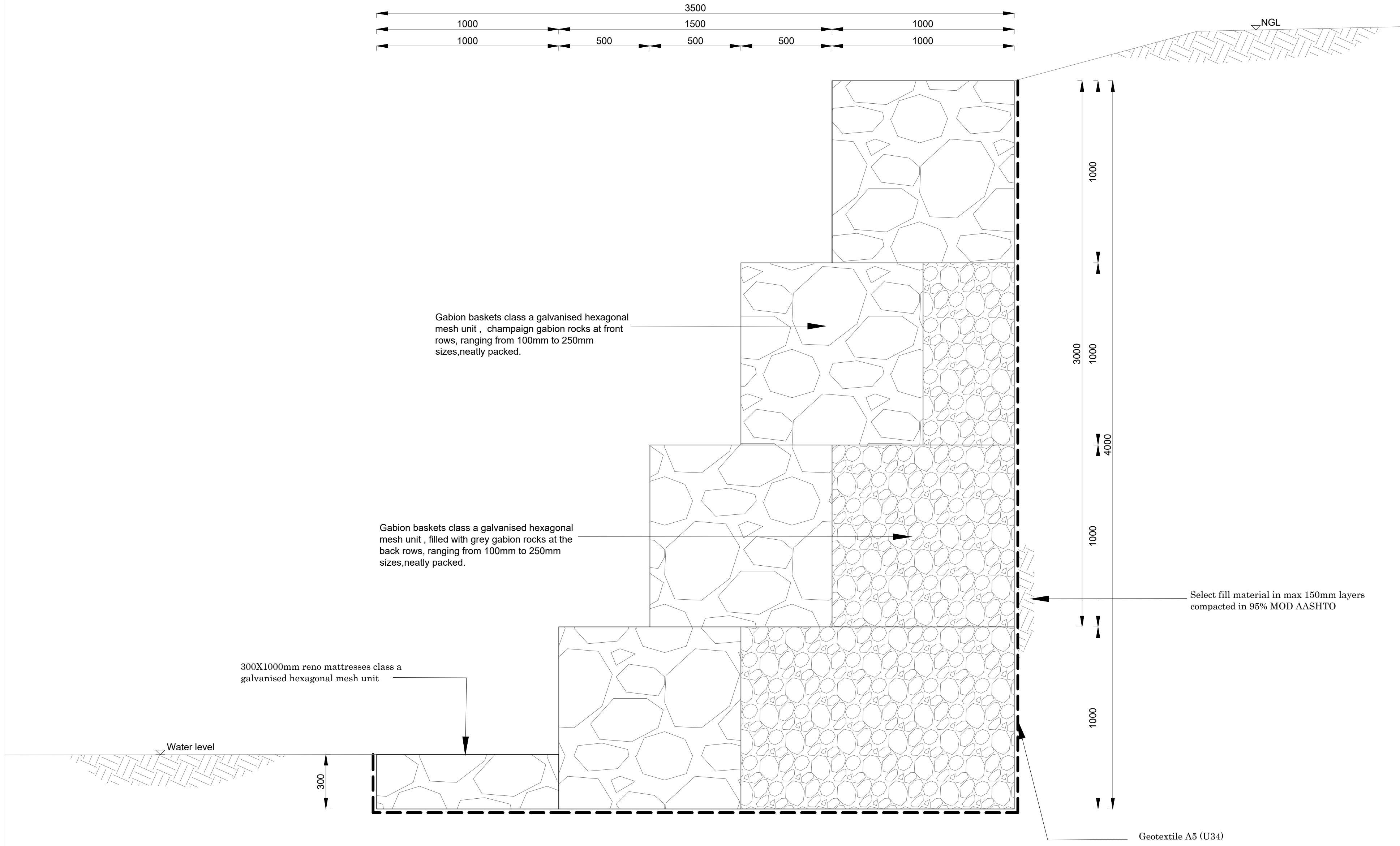
GABION RETAINING WALL SECTION S-S SCALE 1:15
