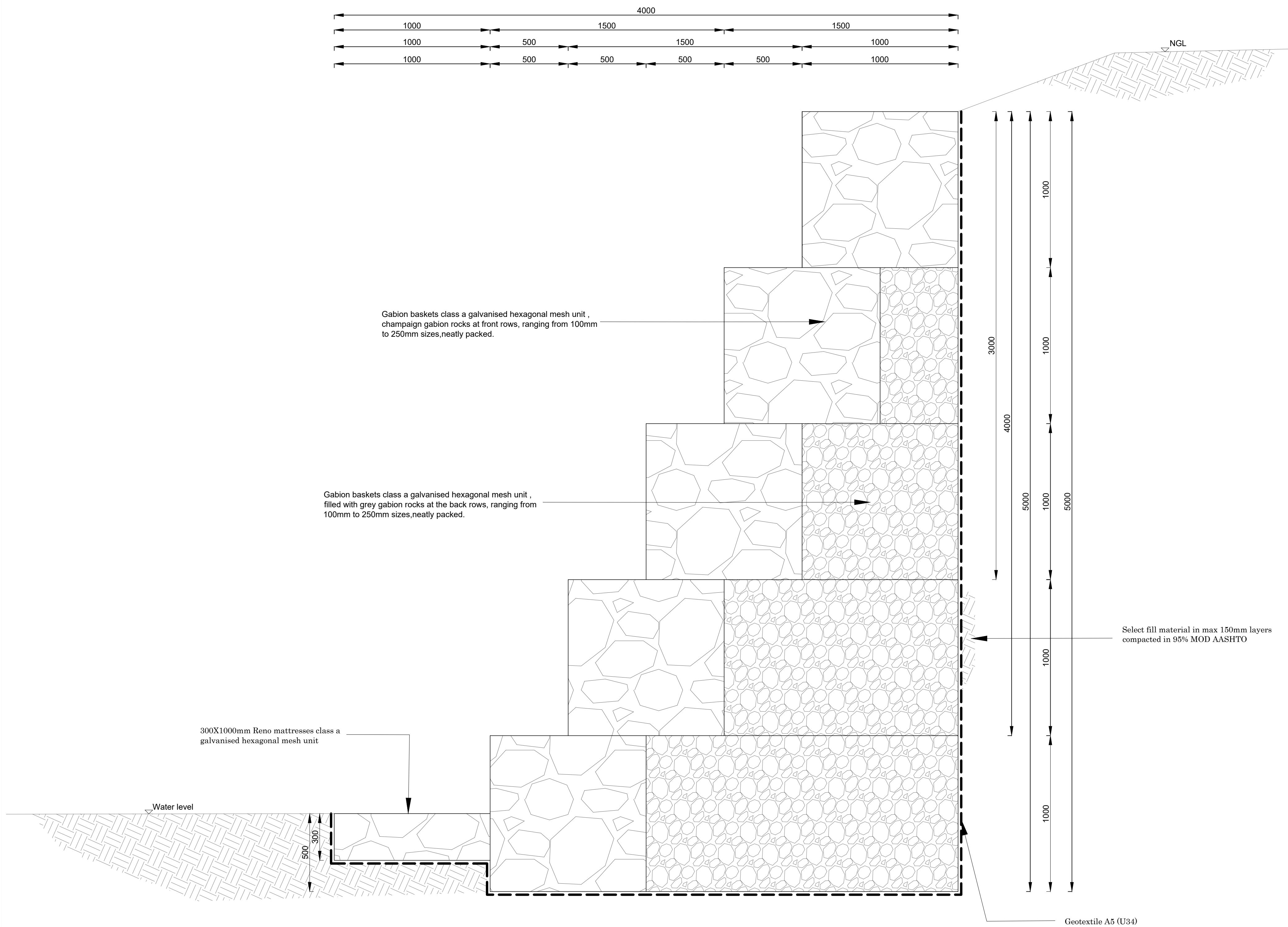
GABION RETAINING WALL SECTION T-T
