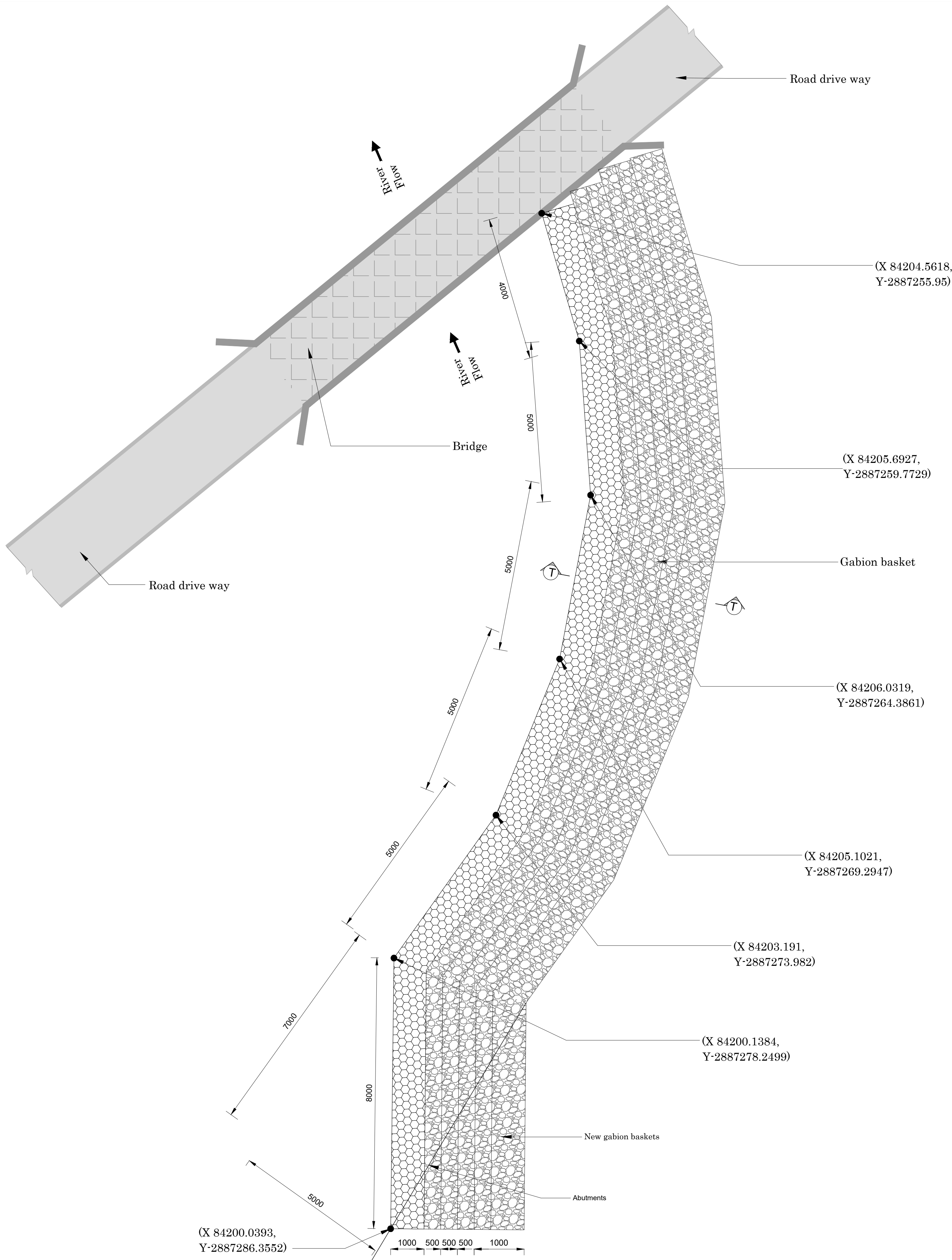
GABIONS RETANING WALL LAYOUT (Water Fall Bridge)
