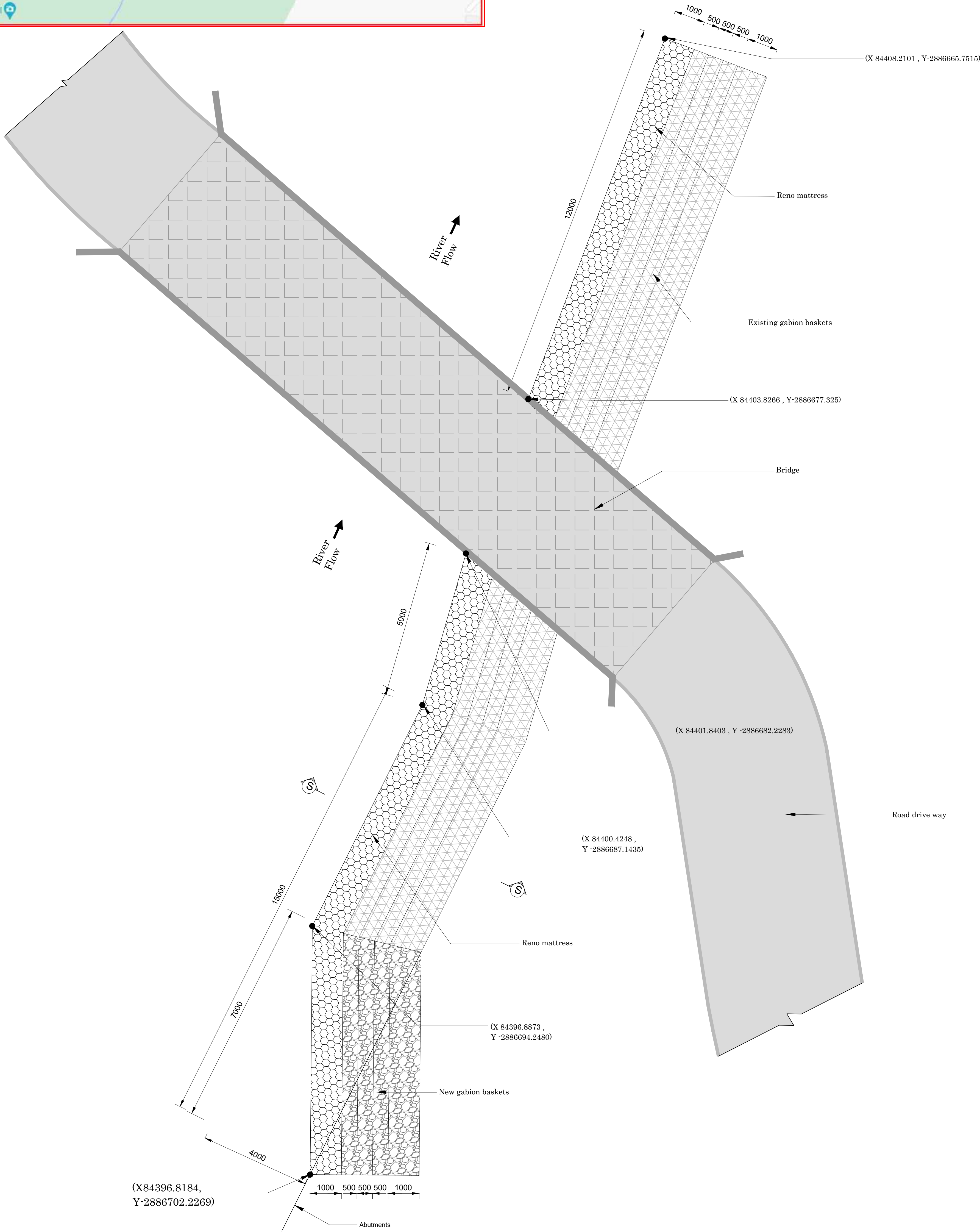
GABIONS RETAINING WALL LAYOUT (Low Level Bridge) SCALE 1:15
