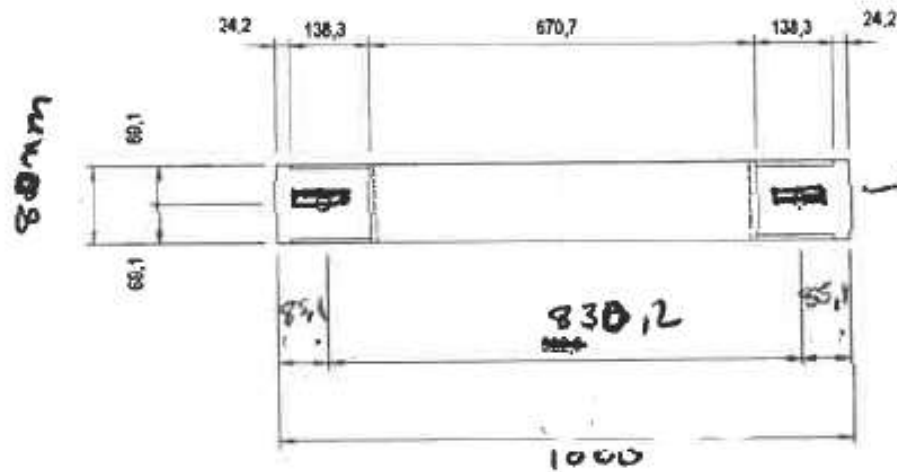
PIPE STRAP DETAIL SCALE 1:10
