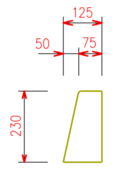
AS PER SANS-927 (FIG.6)
