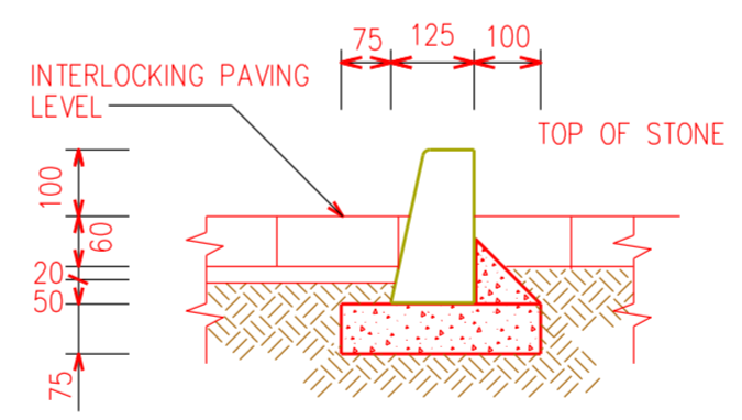
CONCRETE FILLET TO BE PLACED AT 150mm ON BOTH SIDES OF ALL JOINTS FOUNDATION CLASS 20MPa
