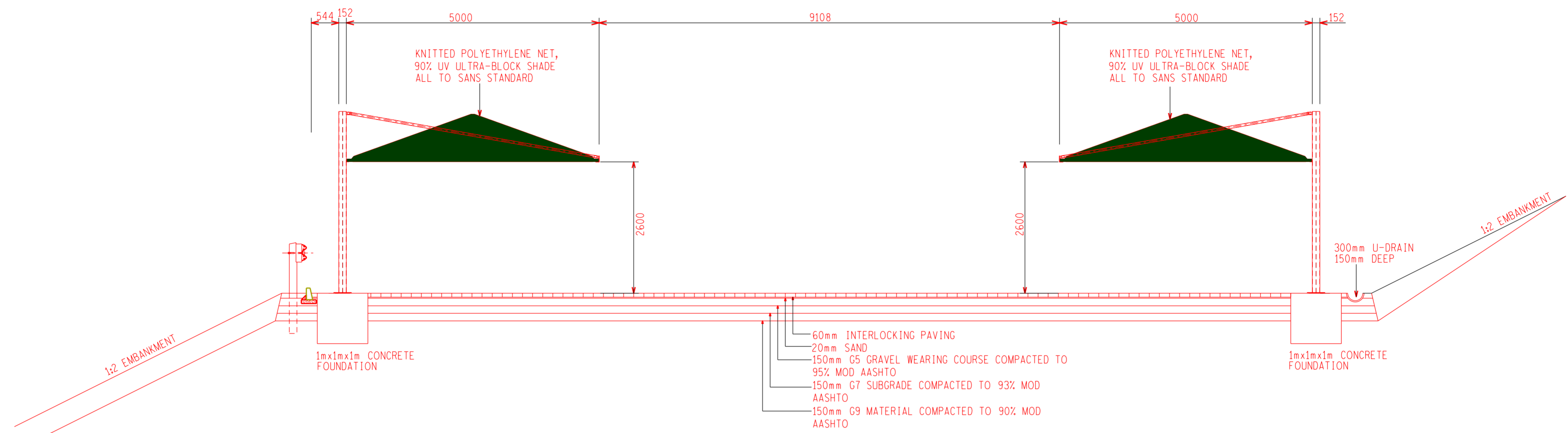
CAR PARKING & CARPORT SECTION A-A 1:60
