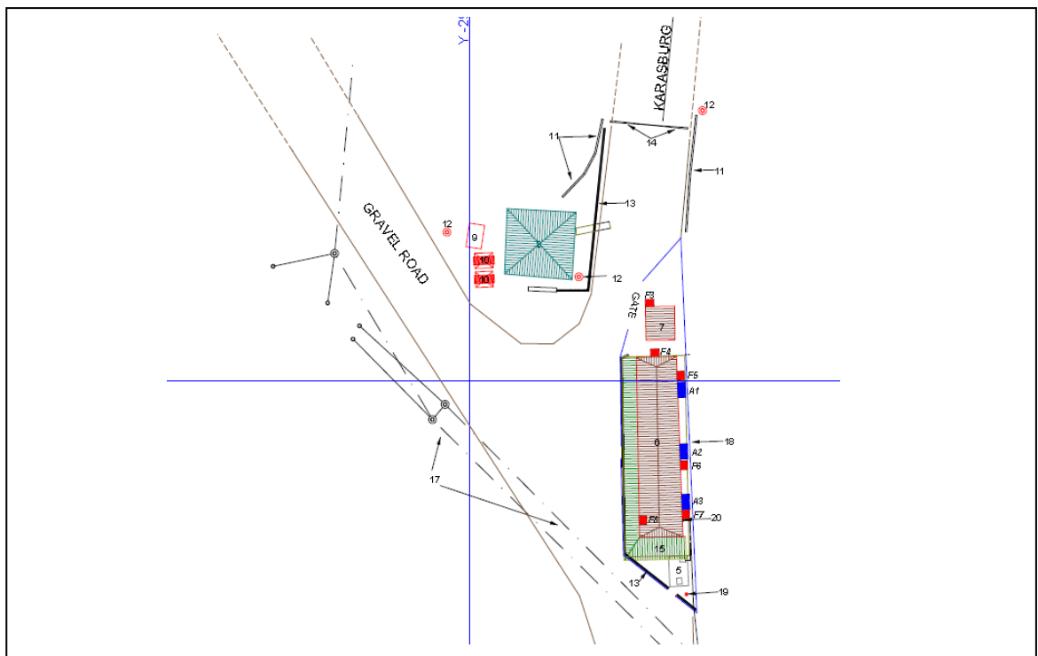
Figure 2.3: Onseepkans Port of Entry: Site Layout
