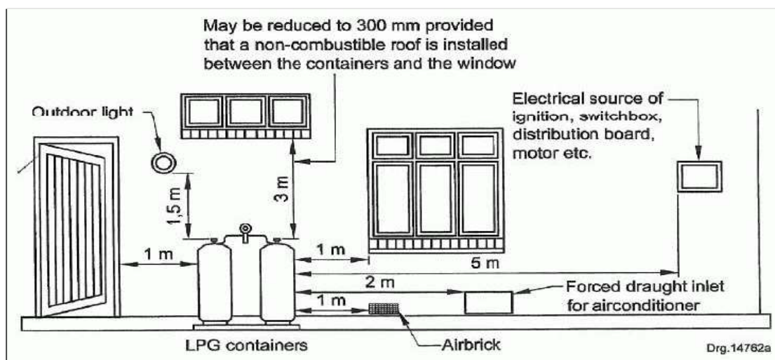
Figure 8: Minimum distances: Electrical, Doors, Windows, and other openings
