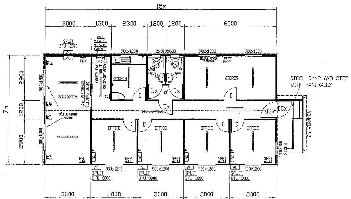
PLAN 105m 2
