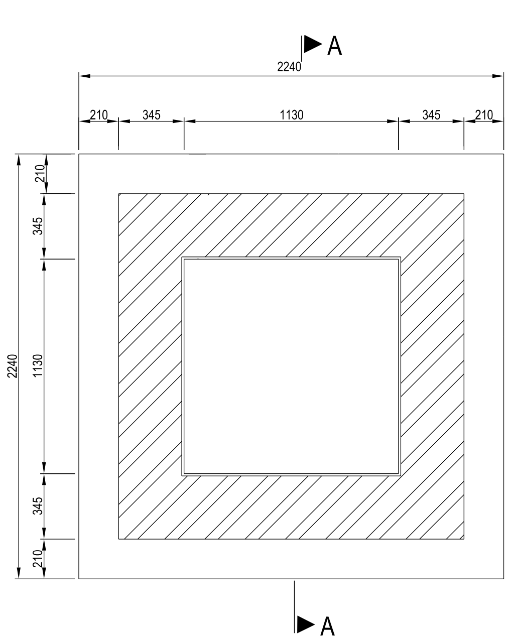
PLAN SCALE 1:20
