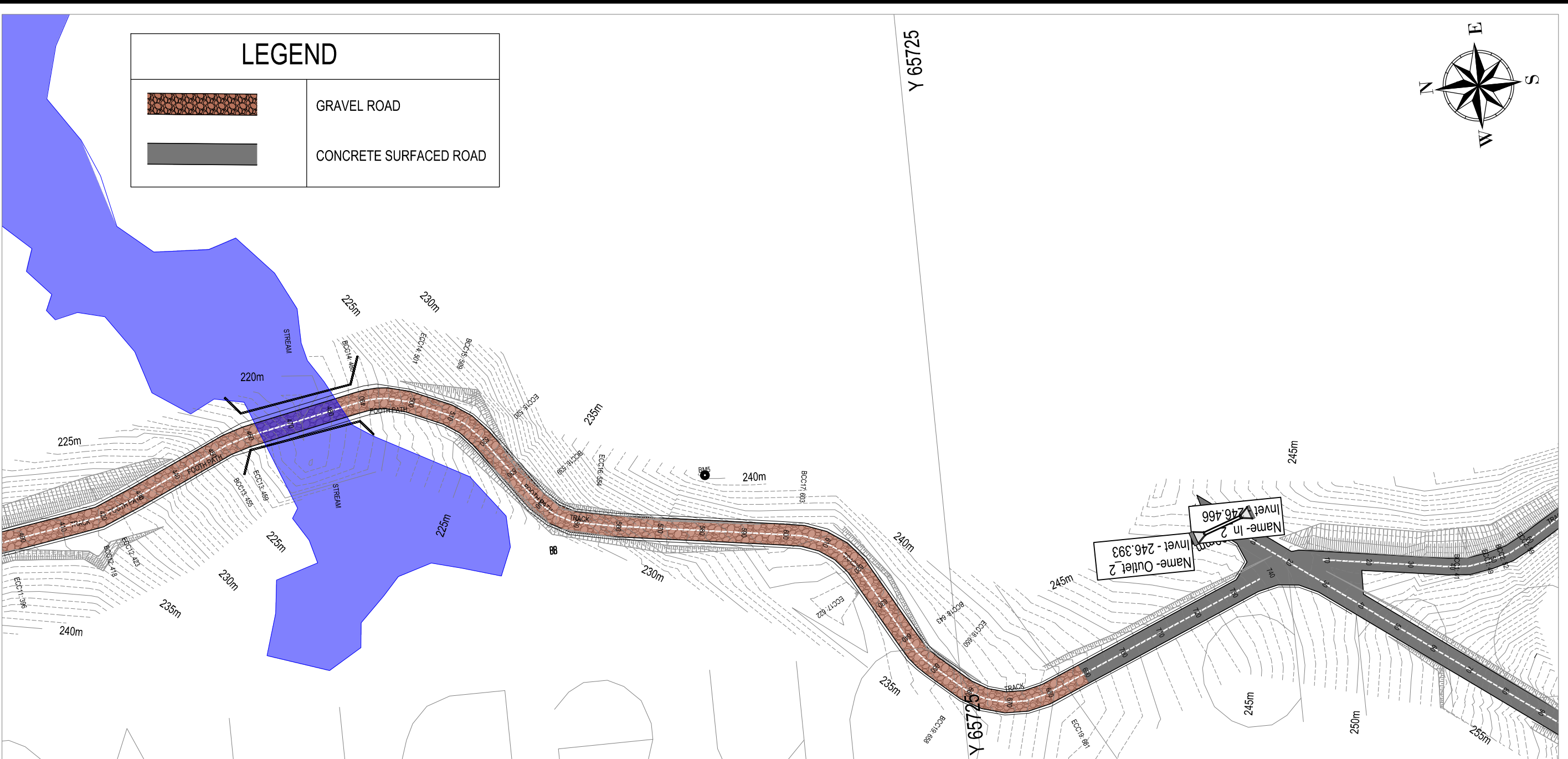
ROAD 1 LAYOUT - CH400 TO END
