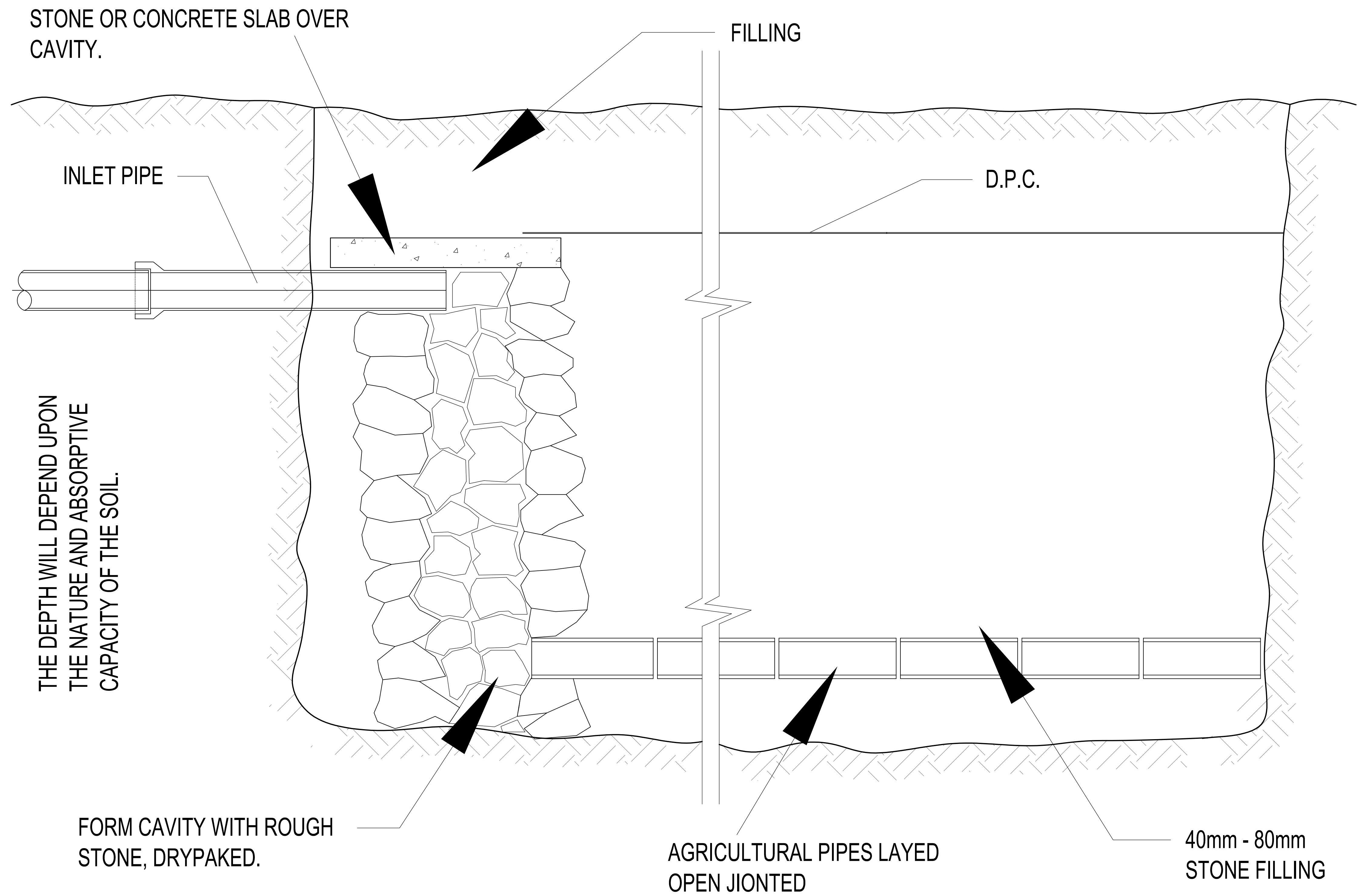
LONGITUDINAL SECTION THRU' FRENCH DRAIN
