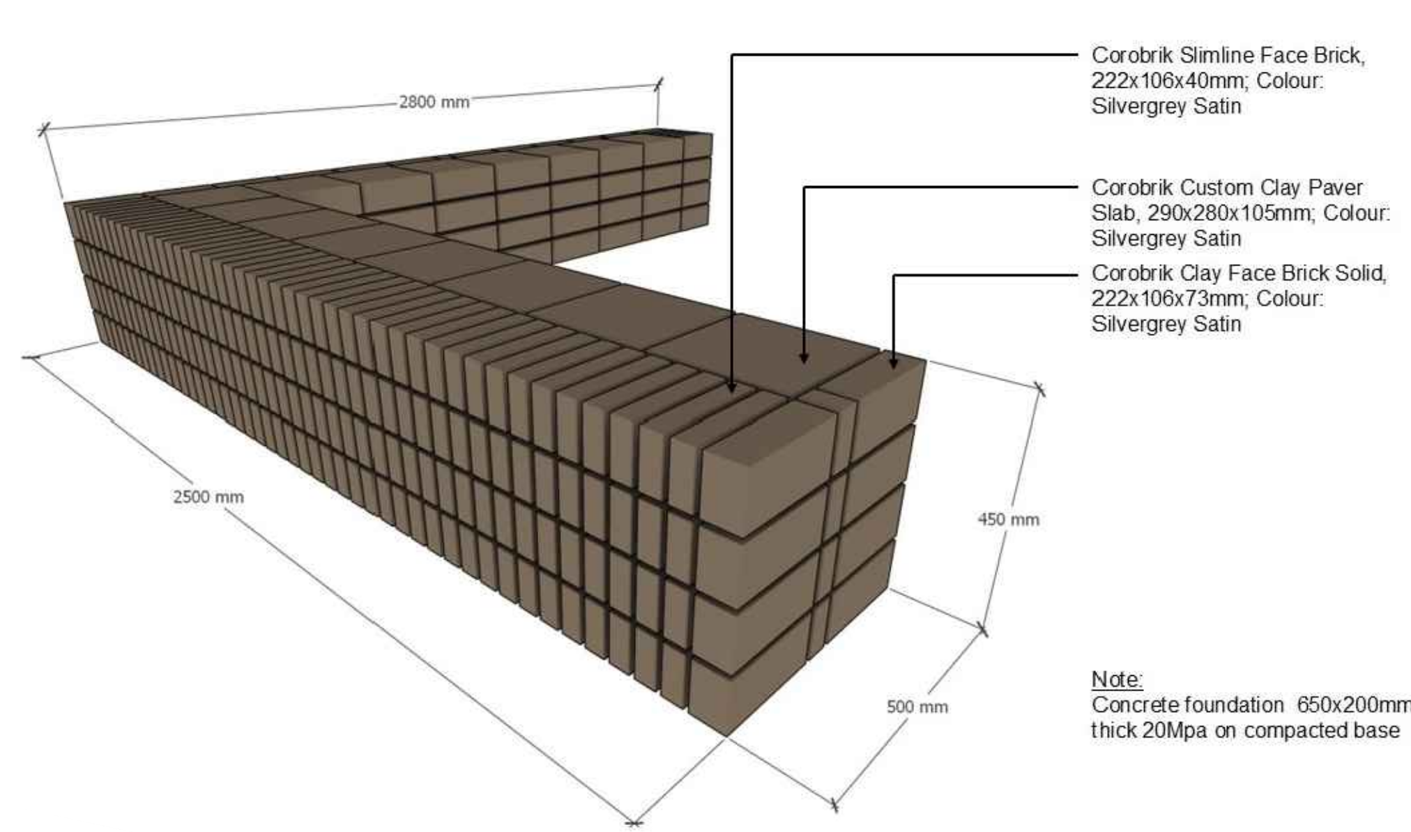
Typical Built Seating wall Detail
