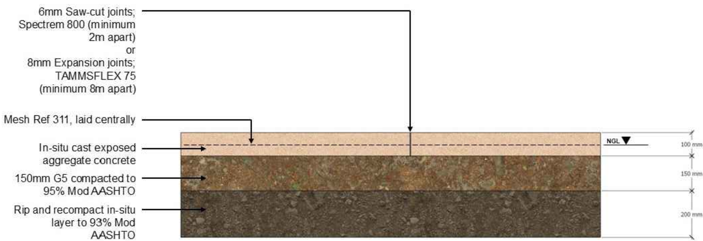
Typical Walkway Section
