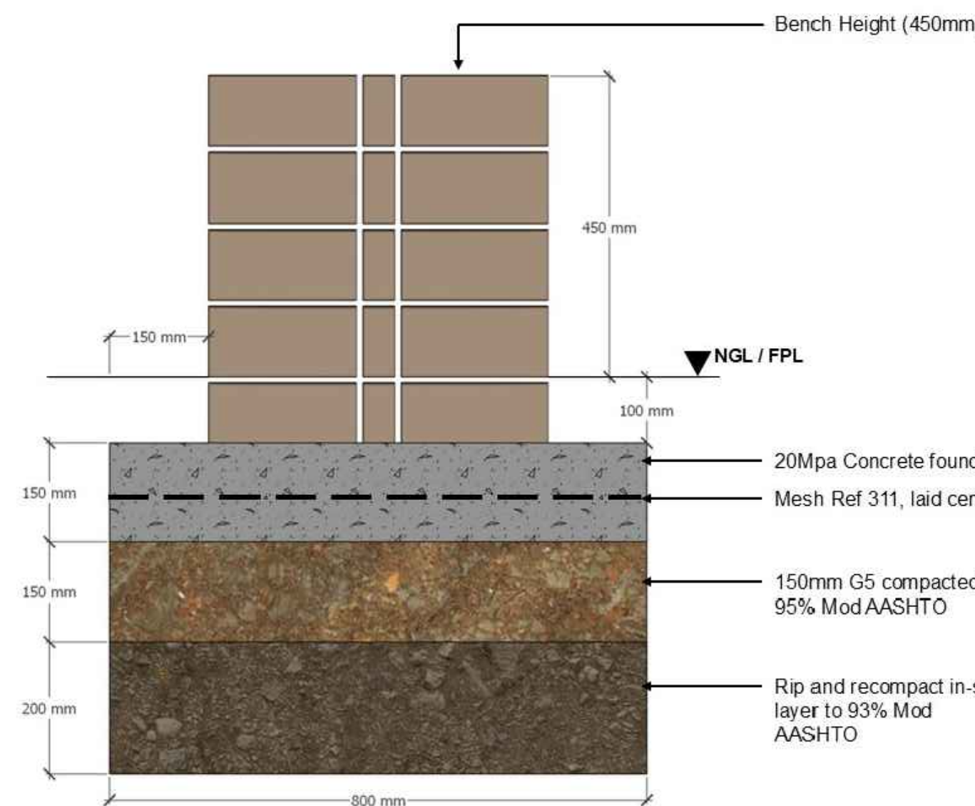
Typical Bench Foundation Section
