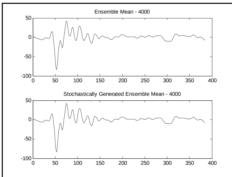
Figure 519.6B-8b. Ensemble and stochastically generated pulse ensemble deterministic component (4000 rnd/min).
