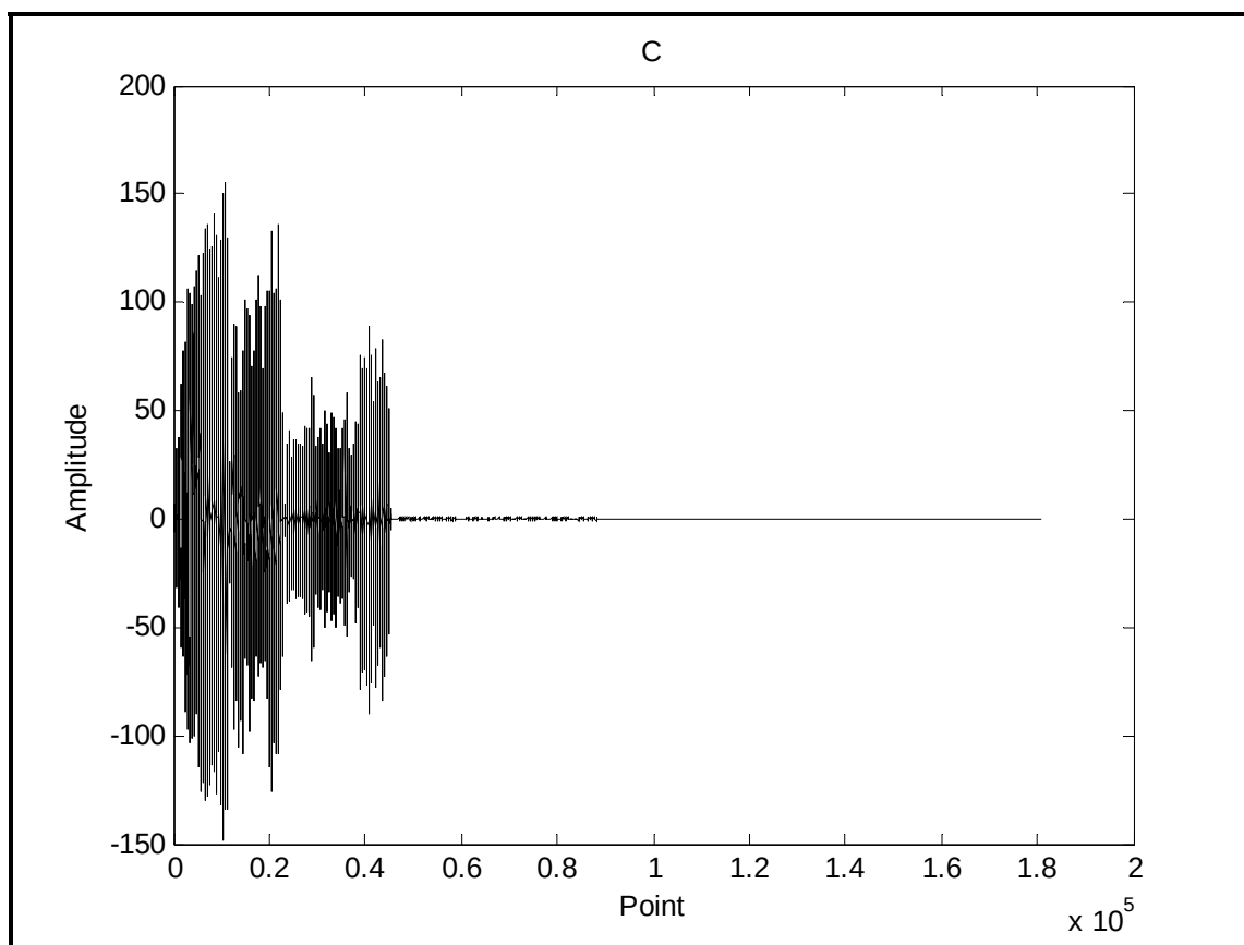
Figure 519.6B-12. db20 Approximation plus decomposition coefficients for the time trace in Figure 519.6B-3.
