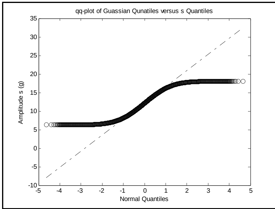
Figure 525A-17. Stationary Vibration q-q plot for s versus Gaussian.
