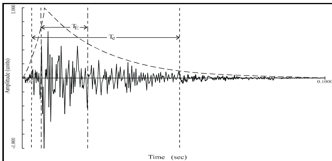
Figure 516.6B-1a. Typical shock time history with envelope, T_E and T_e .
