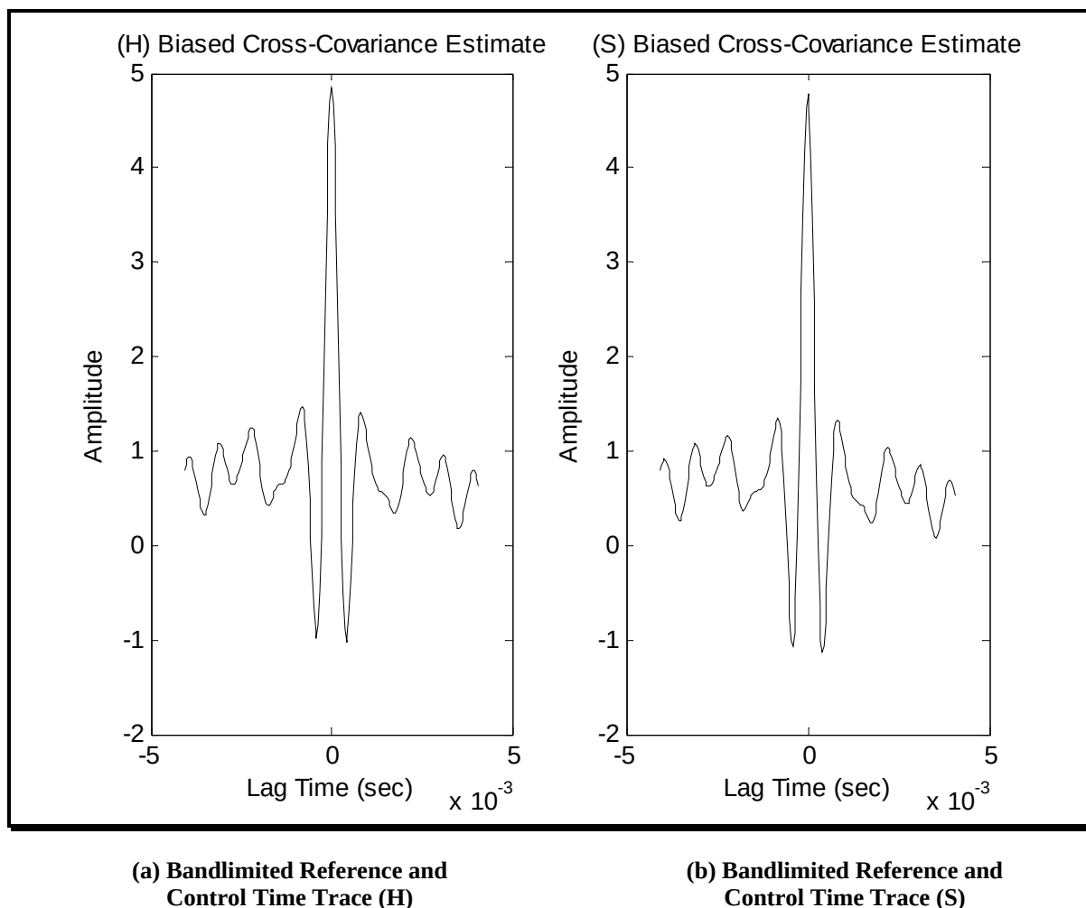
Figure 525A-4. Cross-covariance function estimates between reference and control time traces.
