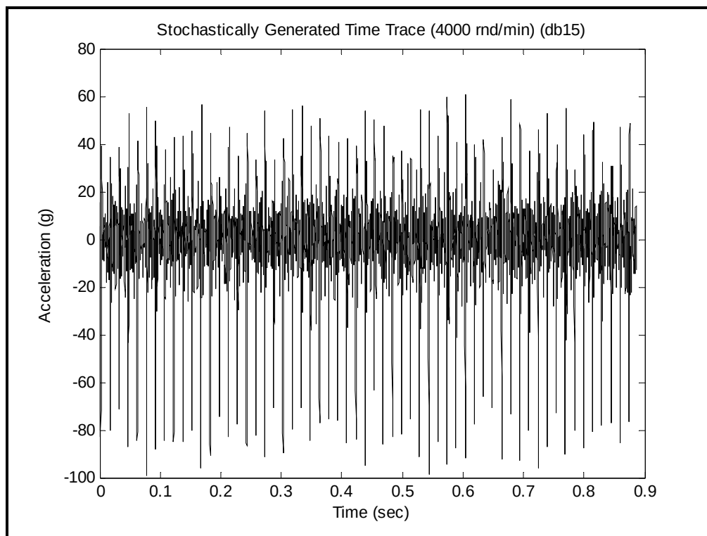
Figure 519.6B-9b. Stochastically generated gunfire shock time trace (4000 rnd/min).
