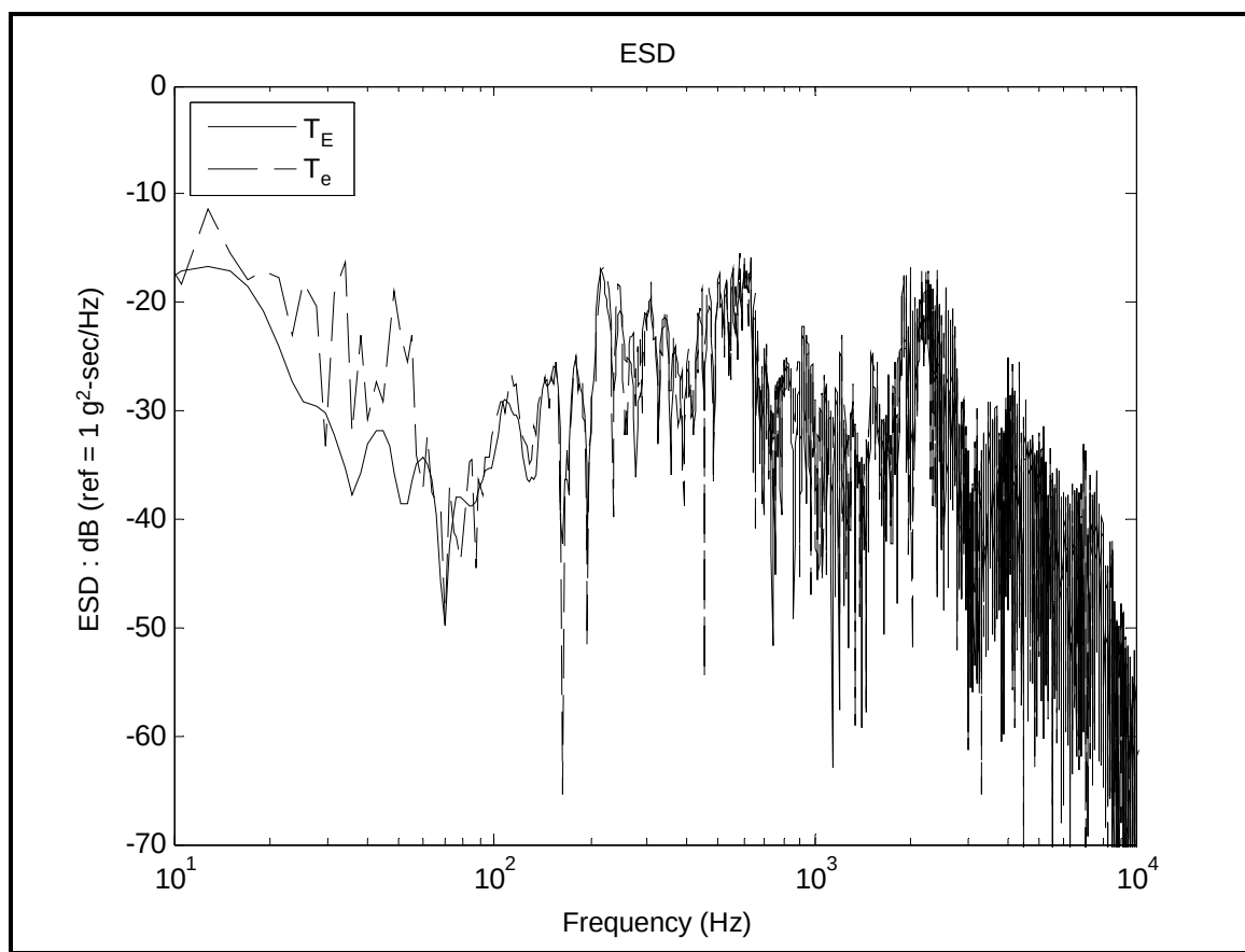
Figure 516.6-7. Energy Spectral Density Estimates over T_E and T_e .
