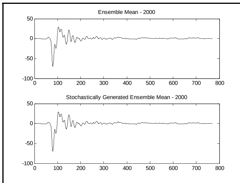
Figure 519.6B-8a. Ensemble and stochastically generated pulse ensemble deterministic component (2000 rnd/min).
