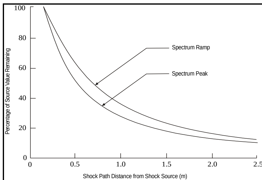
Figure 517.1-9. Shock response spectrum versus distance from pyrotechnic source.
