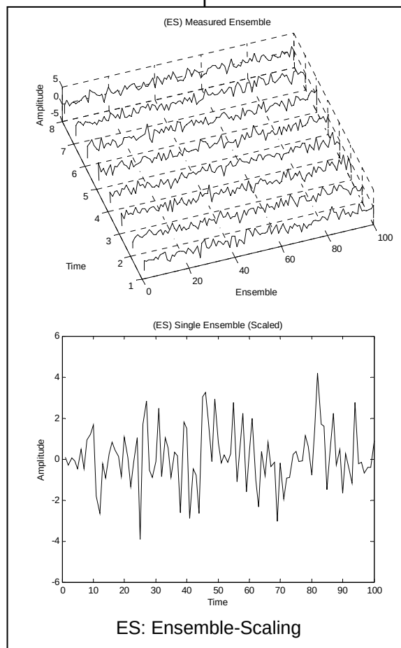
Figure 525-1. Basic TWR test modes as related to time trace scaling.
