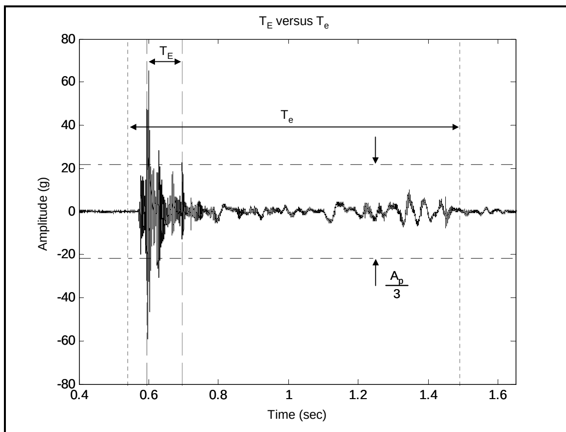
Figure 516.6-3 Shock response time history displaying effective durations T_E and T_e .
