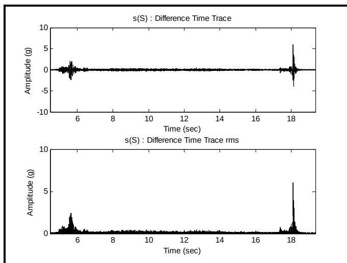
Figure 525A-9b. Difference Exciter (S).
