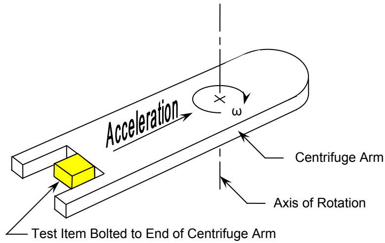
Typical Installation
