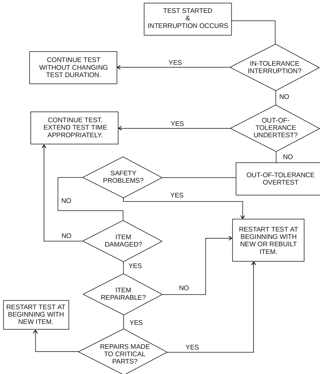
Figure 1-5. Interrupted test cycle logic.
