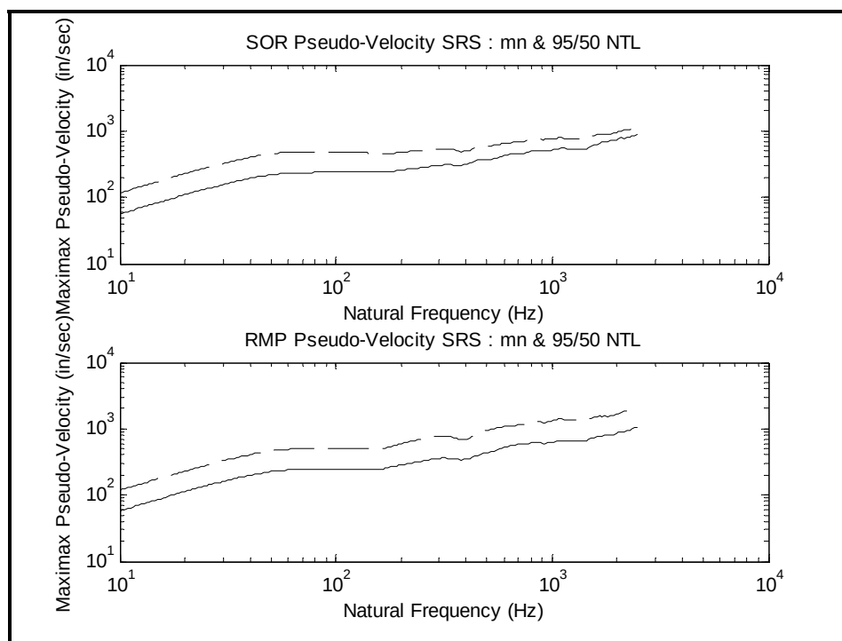
Figure 519.6C-10a. Pseudo-velocity shock response spectra for pulse ensemble with 95/50 NTL
