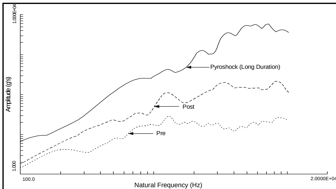
Figure 517.1-5. Acceleration maximax SRS for the pyroshock, pre-pyroshock and post pyroshock.
