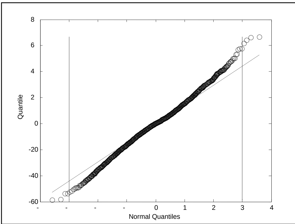
Figure 519.6B-7b. qq-Plot for composite random component decomposition 4000 rnd/min.
