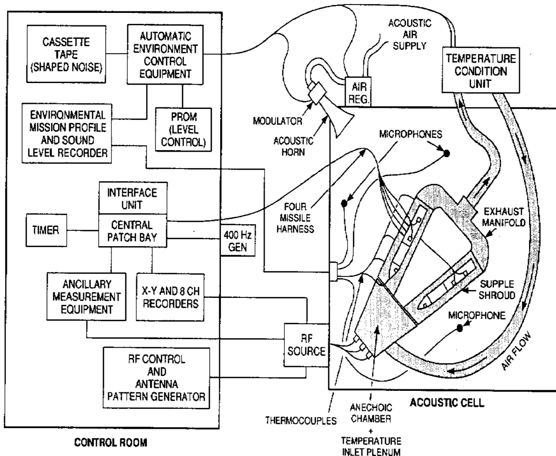
Figure 523.3A-7. Typical arrangement of test apparatus.
