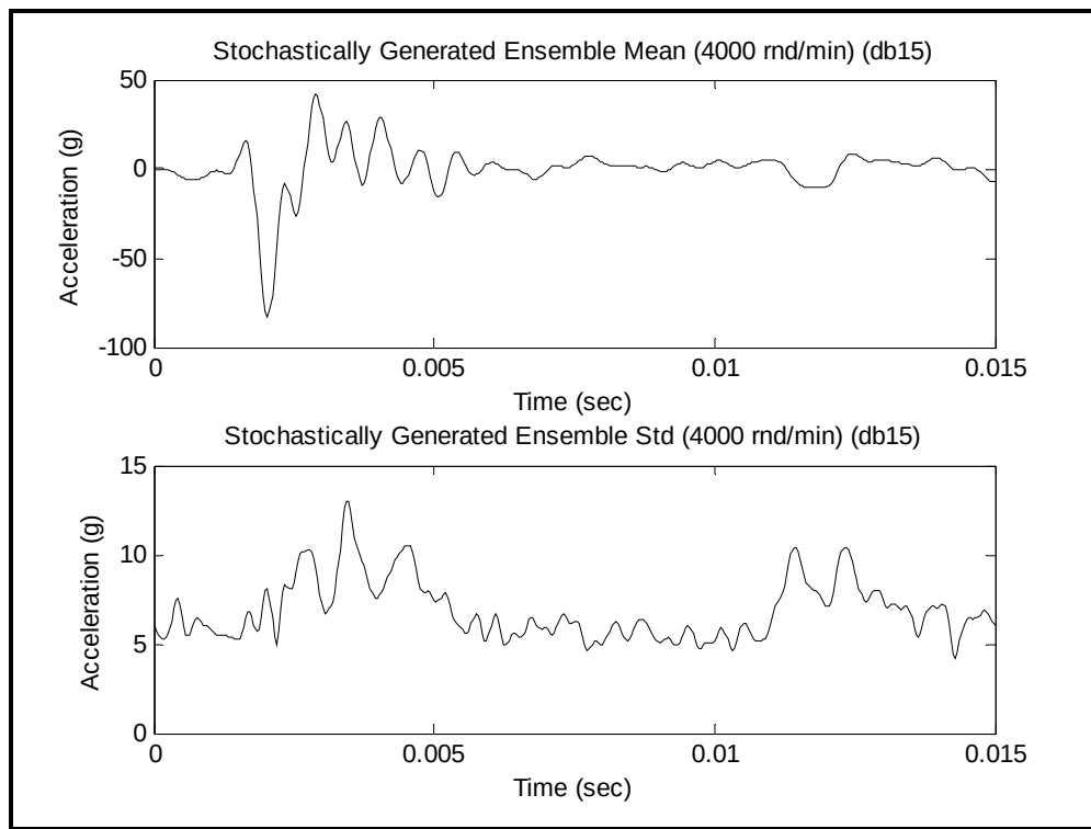
Figure 519.6B-8d. Ensemble and stochastically generated pulse ensemble random component standard deviation (4000 rnd/min)
