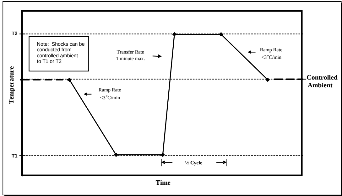
Figure 503.5-1. Single shock (1/2 cycle).
