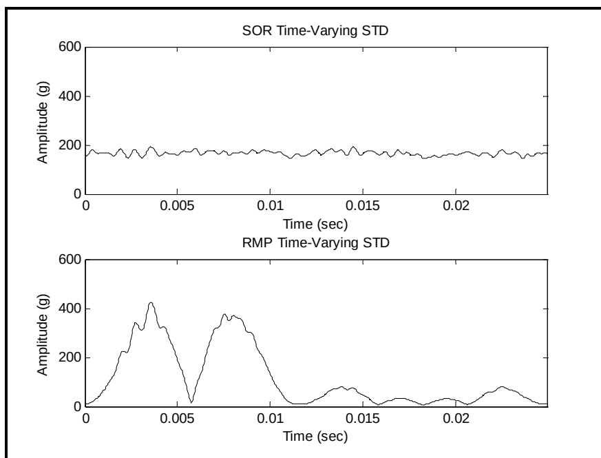
Figure 519.6C-9b. Pulse ensemble statistics - standard deviation of random component r(t) .
