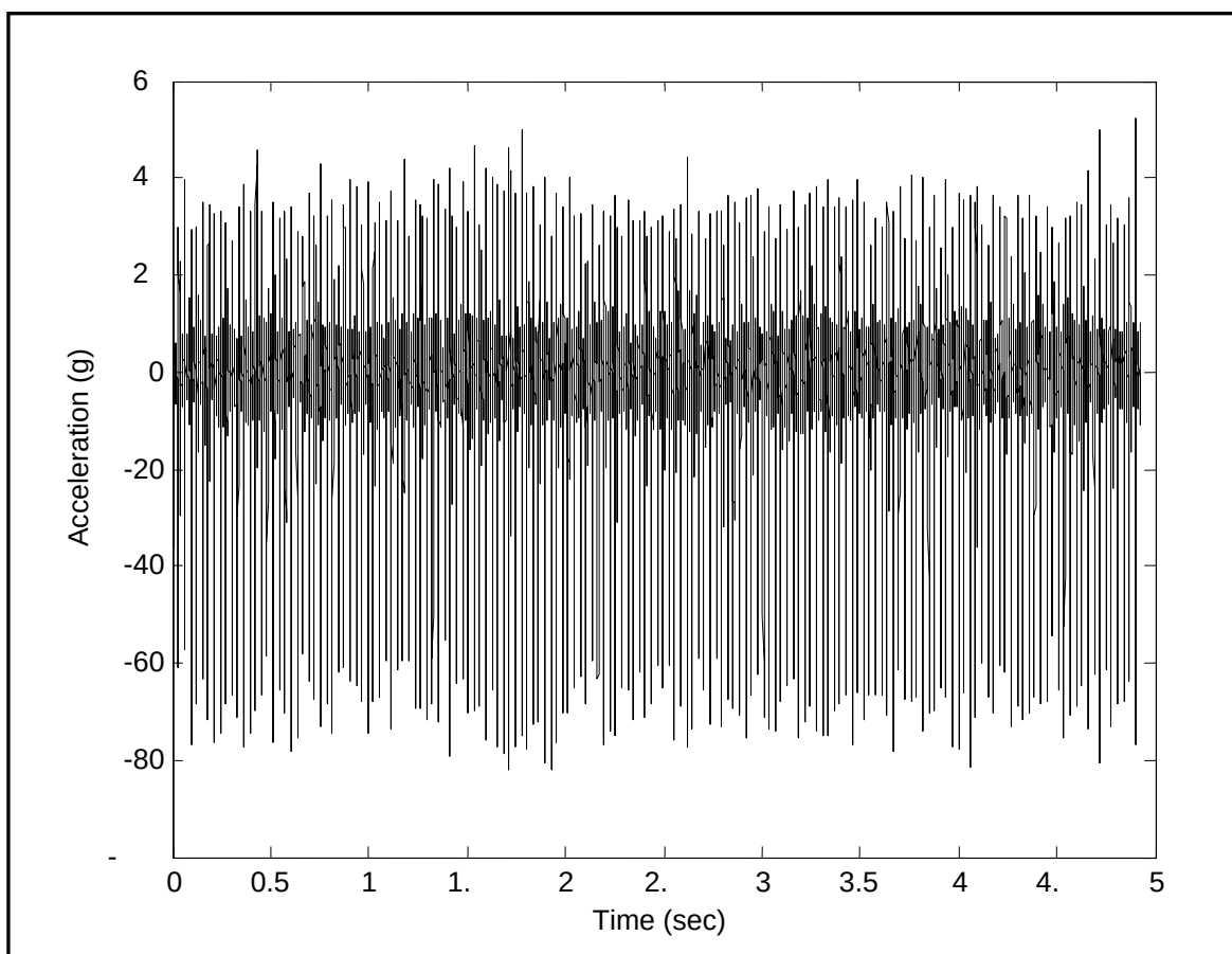
Figure 519.6B-5a. Concatenated measured gunfire shock time trace (2000 rnd/min).
