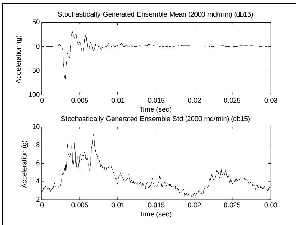
Figure 519.6B-8c. Ensemble and stochastically generated pulse ensemble random component standard deviation (2000 rnd/min).
