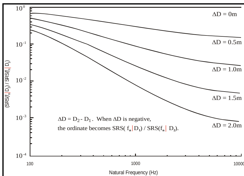
Figure 517.1-7. Empirical scaling relationship for shock response spectrum as a function of the distance from the pyrotechnic source.
