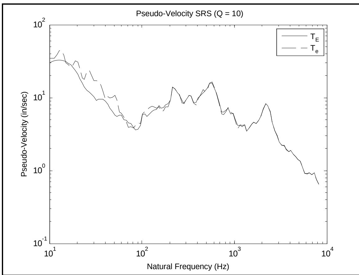
Figure 516.6-6. Pseudo-Velocity SRS over T_E and T_e for Dynamic Quality Factor Q of 10.
