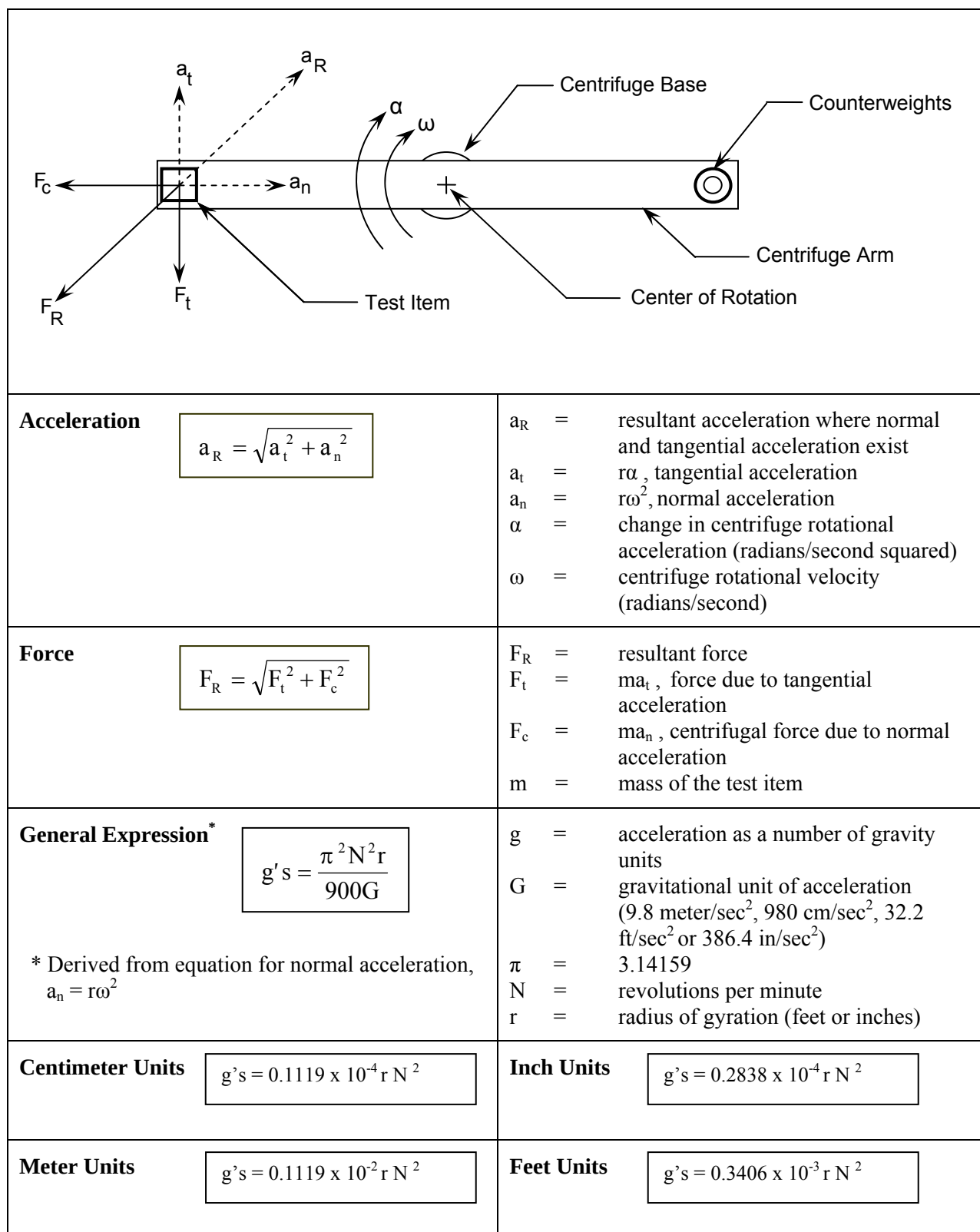
Figure 513.6A-4. Basic forces imposed on test item due to accelerations produced by centrifuge.
