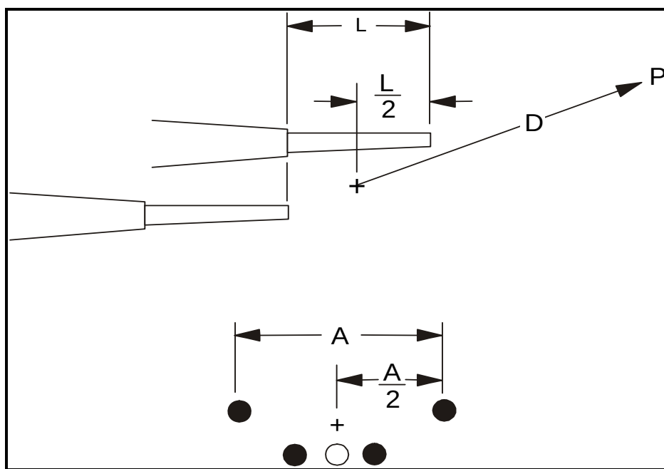
FIGURE 519.6D-3. Multiple guns, closely grouped.
