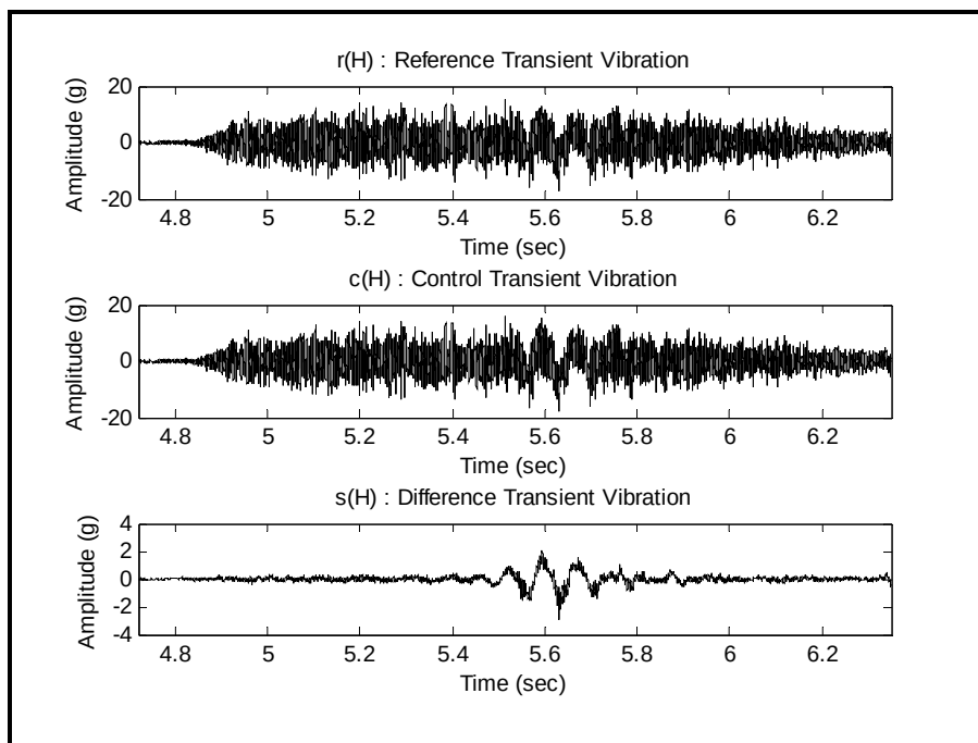
Figure 525A-10. Transient vibration time traces - r, c, and s.
