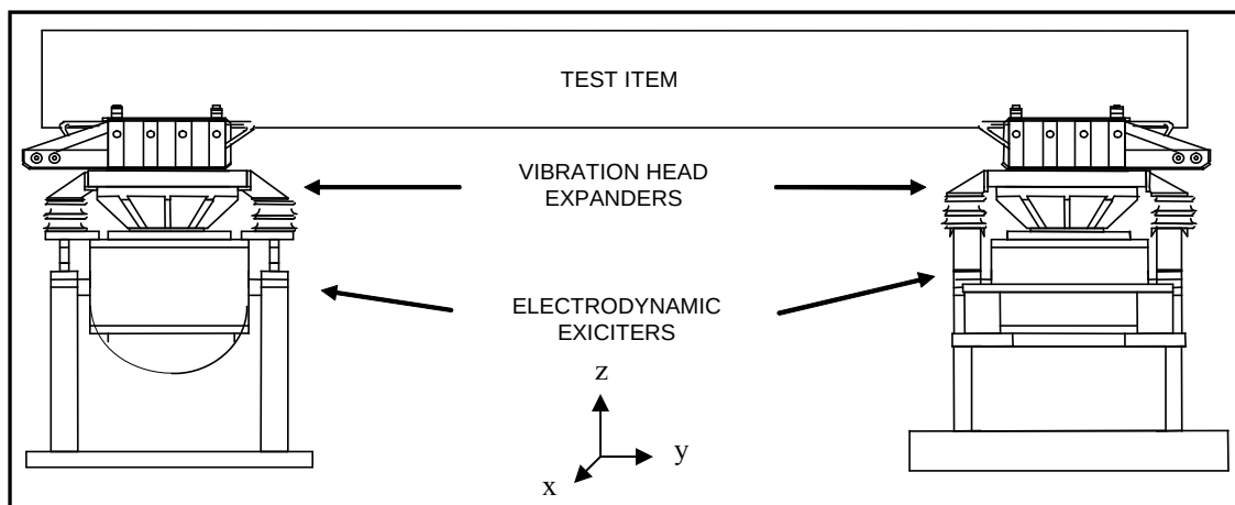
Figure 527-2. MESA - Two exciter test setup
