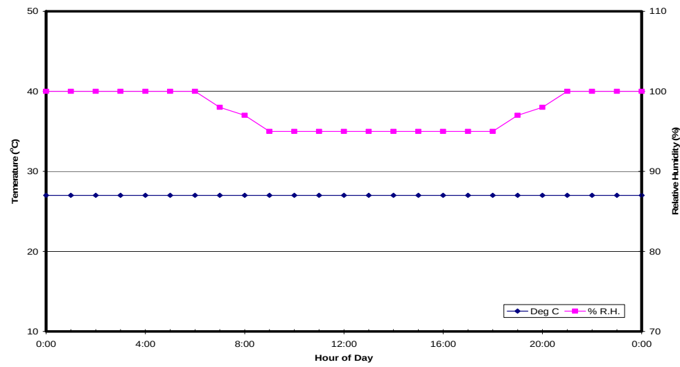
Figure 507.5-1. Induced Cycle B1 – Storage and transit.
