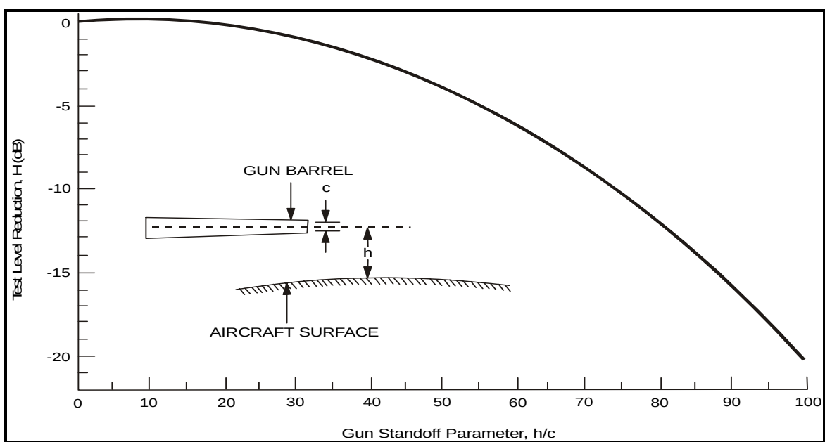
FIGURE 519.6D-4. Test level reduction due to gun standoff parameter.
