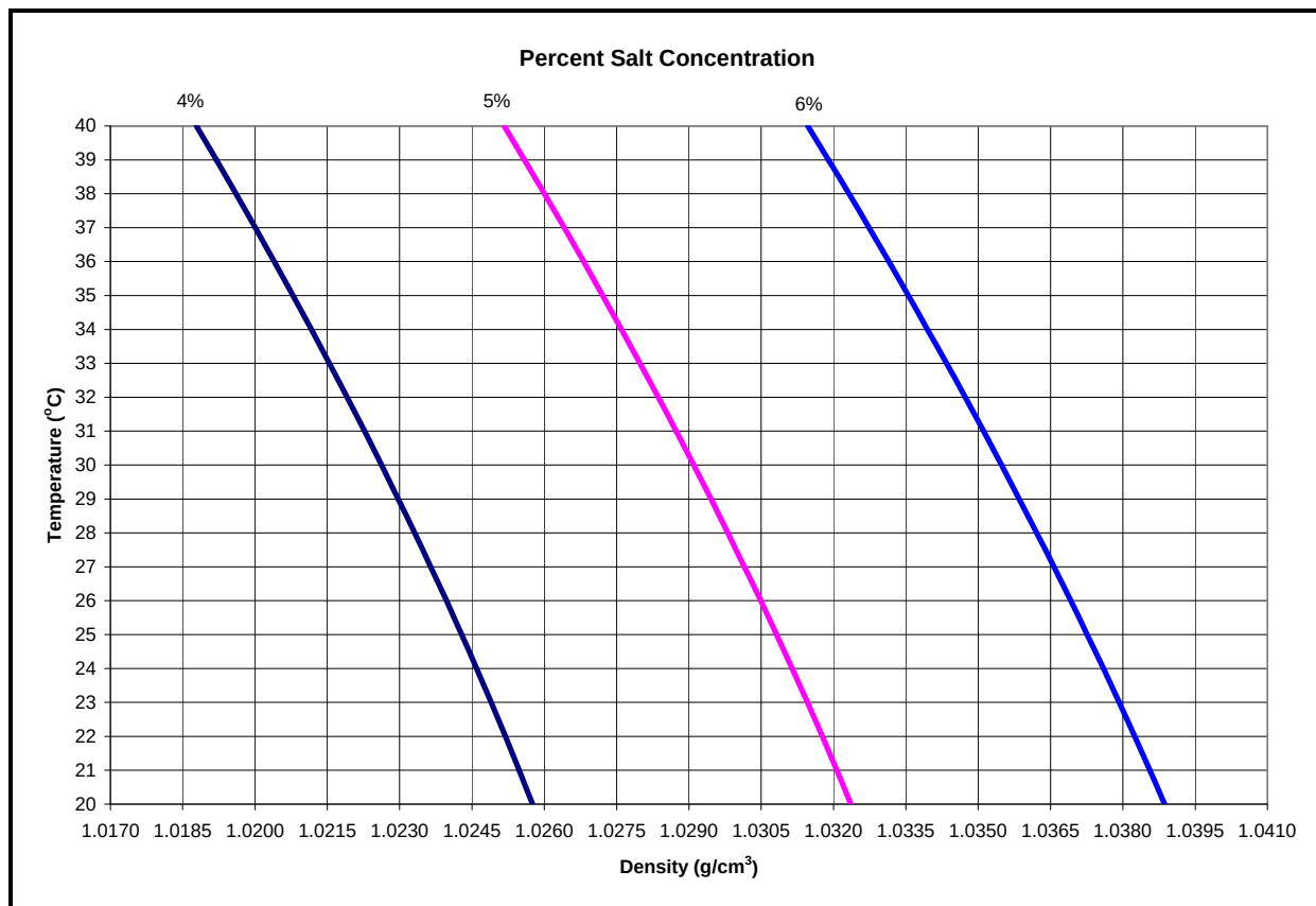
Figure 509.5-3. Variations of density of salt (NaCl) solution with temperature. 1
