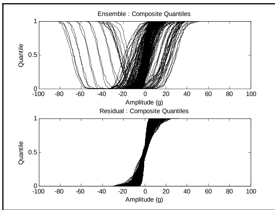
Figure 519.6E-1. Time increment composite cumulative probability distribution function for ensemble and residual.
