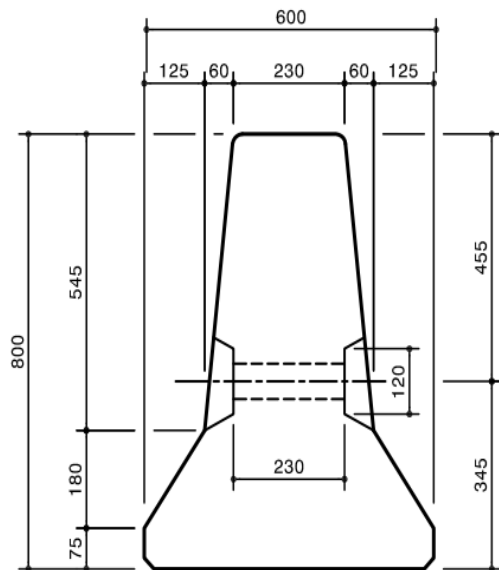
Figure 1: cross section – new Jersey Barrier
