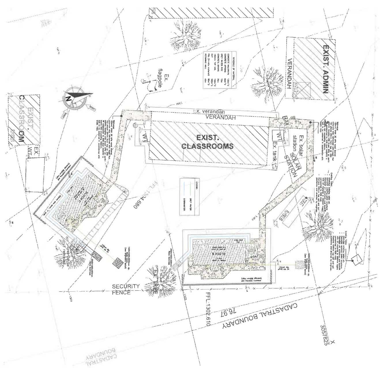
HARD SURFACES, STORMWATER AND GREY WATER LAYOUT PLAN
