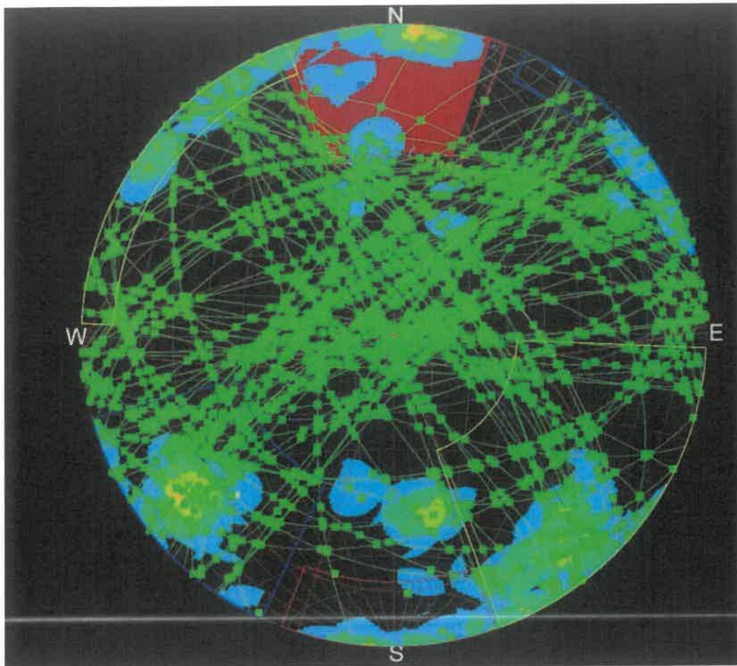
Figure 7: Kinematic analysis
