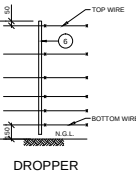
DROPPER
