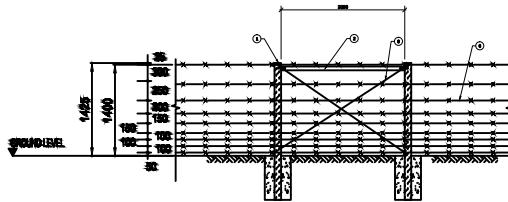
STRAINING POST DETAIL
