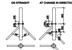
DETAIL OF INTERMEDIATE POSTS SCALE 1:20
