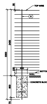
INTERMEDIATE POST
