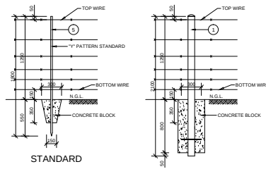
INTERMEDIATE POST
