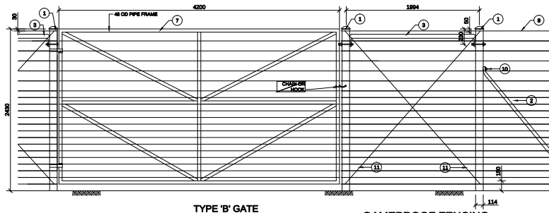
GAMEPROOF FENCING
