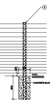
INTERMEDIATE POST
