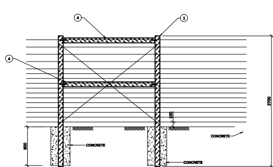
GATE, CORNER OR STRAINING POST
