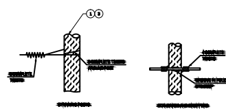
FASTENING OF BARBED WIRE TO DROPPERS
