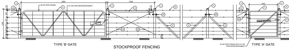
STOCKPROOF FENCING
