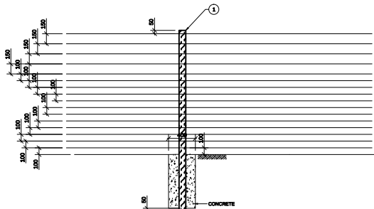
STRAINING POST
