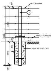
INTERMEDIATE POST
