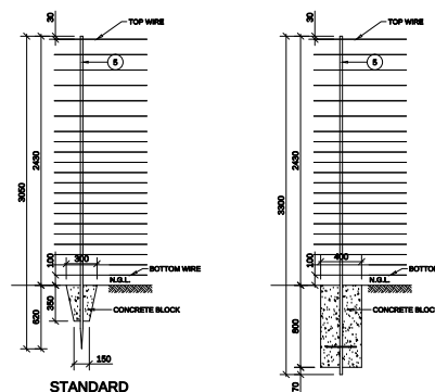
INTERMEDIATE POST
