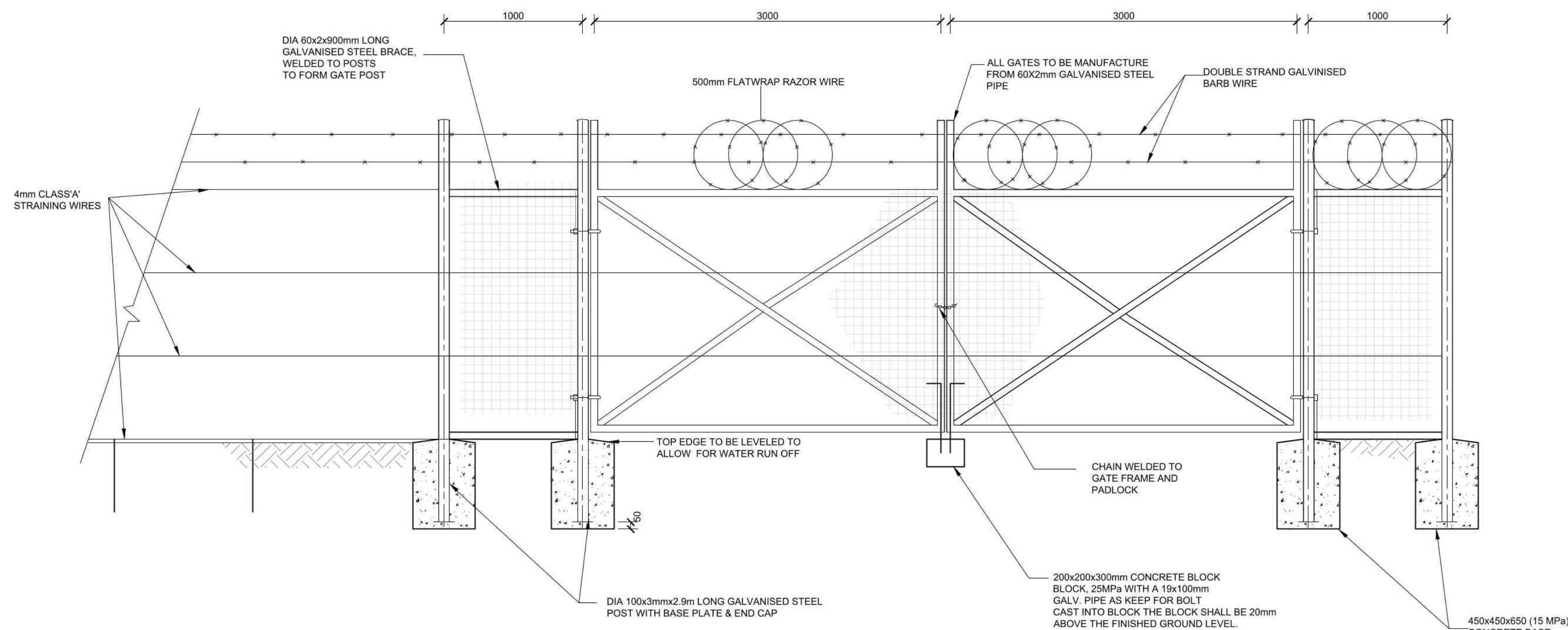
ELEVATION ON VEHICLE GATE ON EXTERNAL FENCE SCALE 1:25
