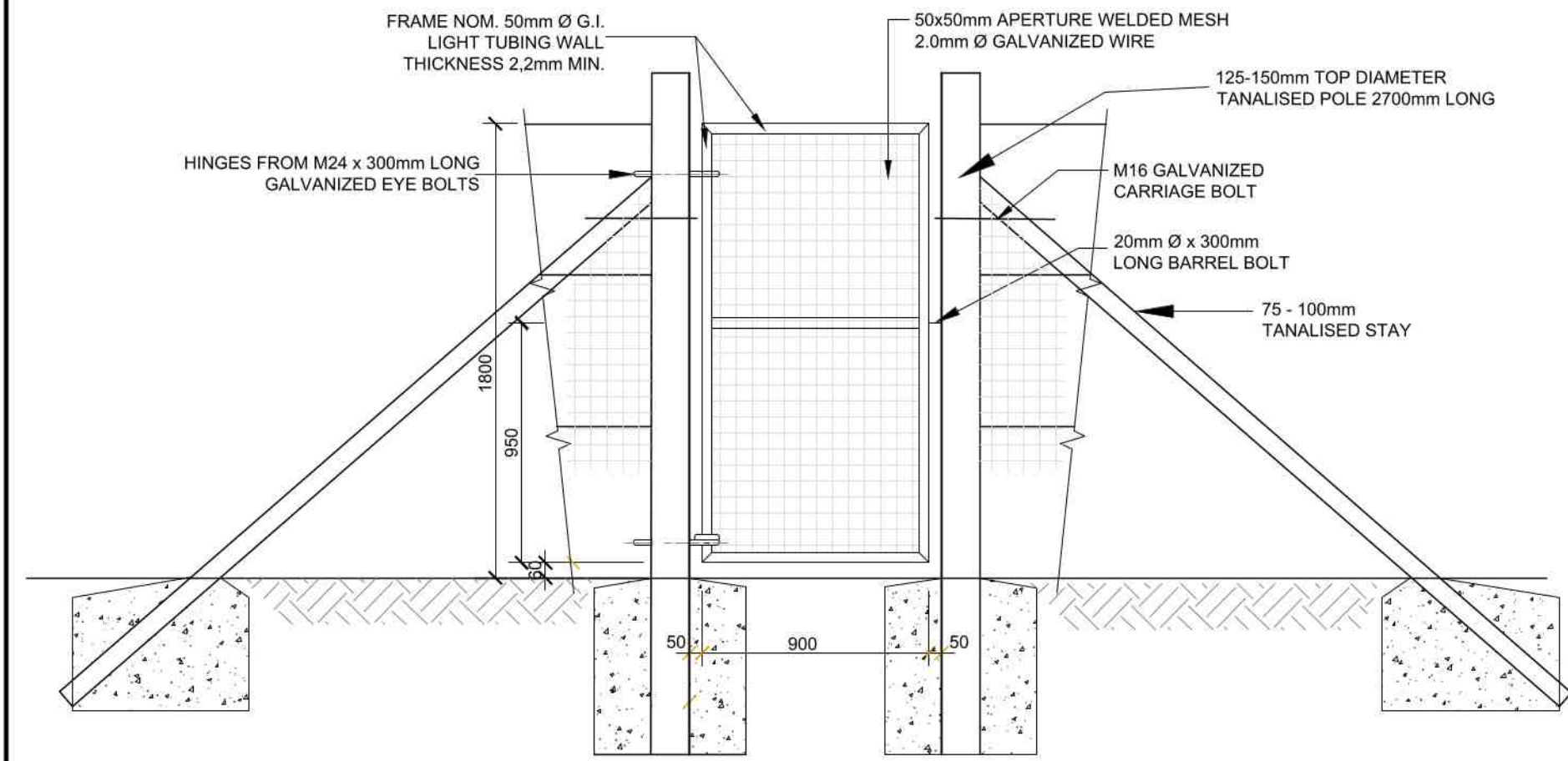
DETAILS OF PEDESTRIAN GATE FOR 1.8m SECURITY FENCE FOR GRADE R SCALE 1:25
