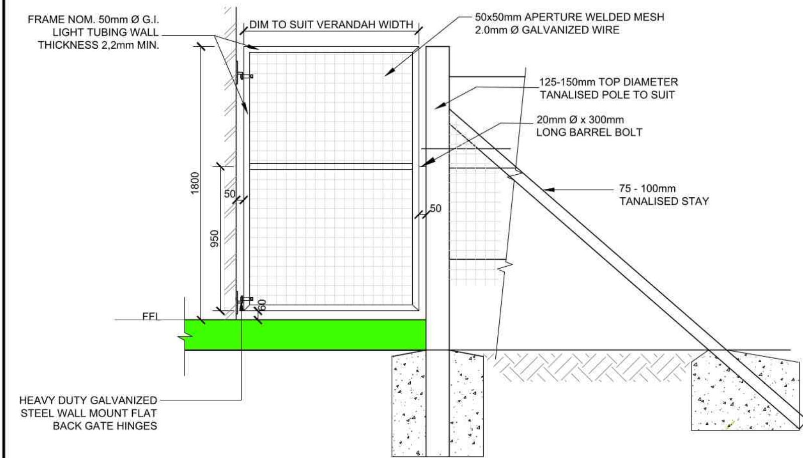
DETAILS OF VERANDAH GATE FOR GRADE R SCALE 1:25
