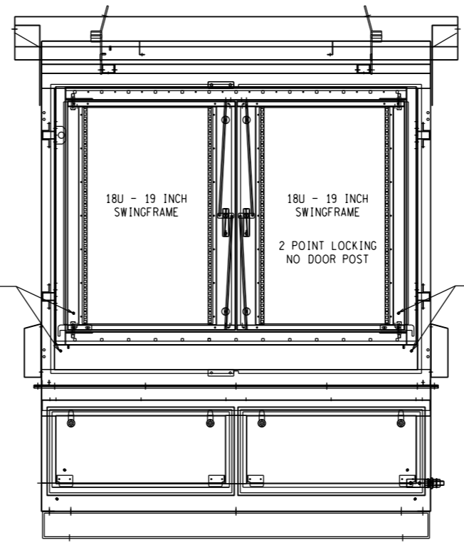
FRONT VIEW OUTER DOORS REMOVED 18U SWINGFRAME
