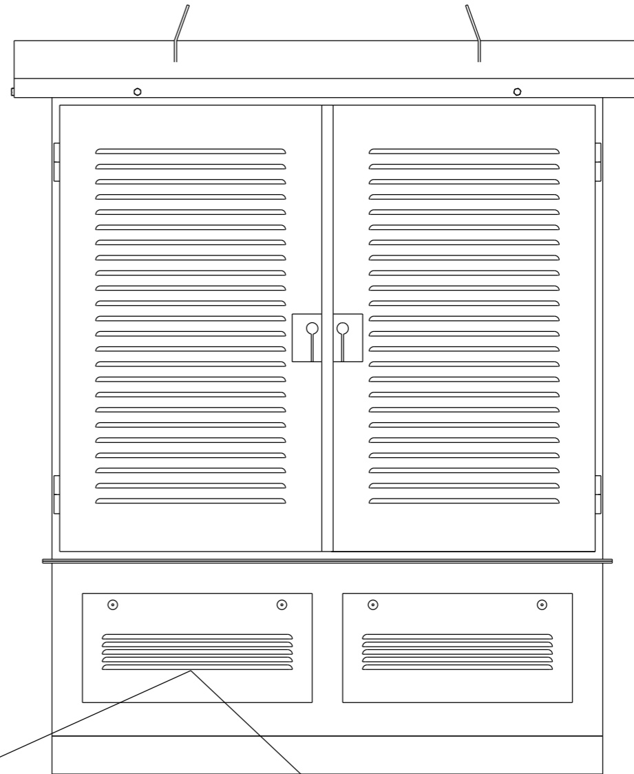
FRONT VIEW SCALE 1:6
