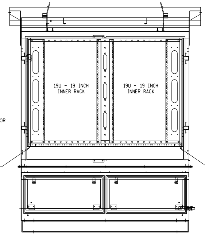
FRONT VIEW OUTER DOORS AND SWING FRAME REMOVED
