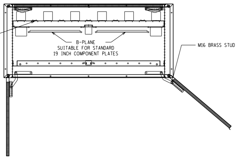
SECTIONAL TOP VIEW (OPEN DOORS AND SWING FRAMES)
