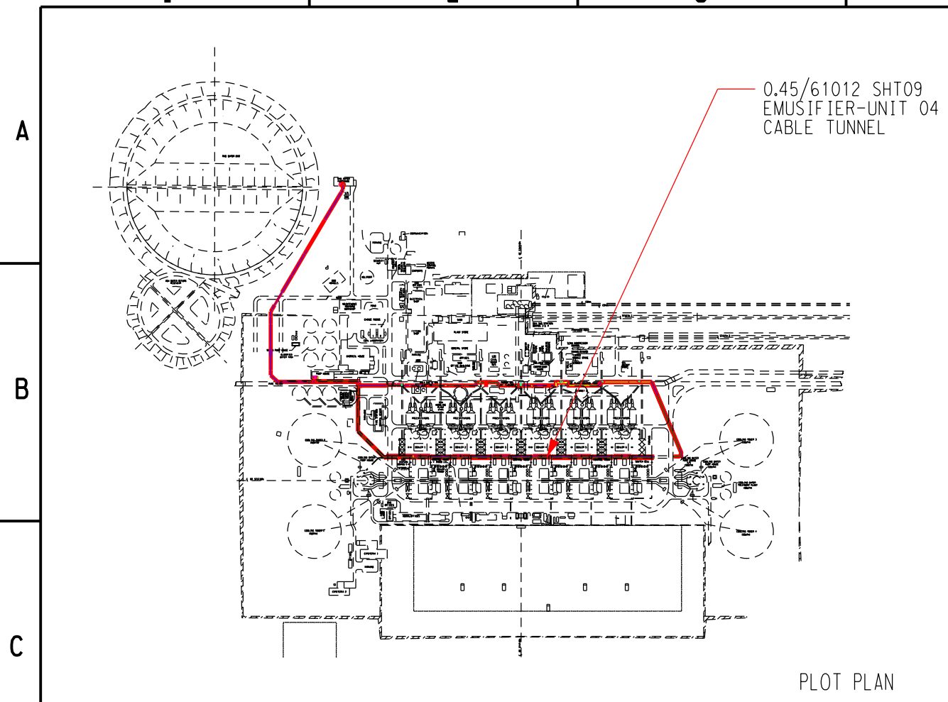
PLOT PLAN
