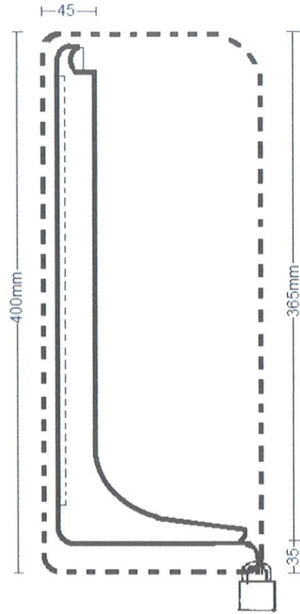
SECTION SIDE VIEW
