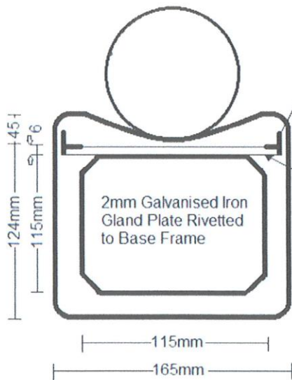
TOP VIEW (COVER REMOVED)
