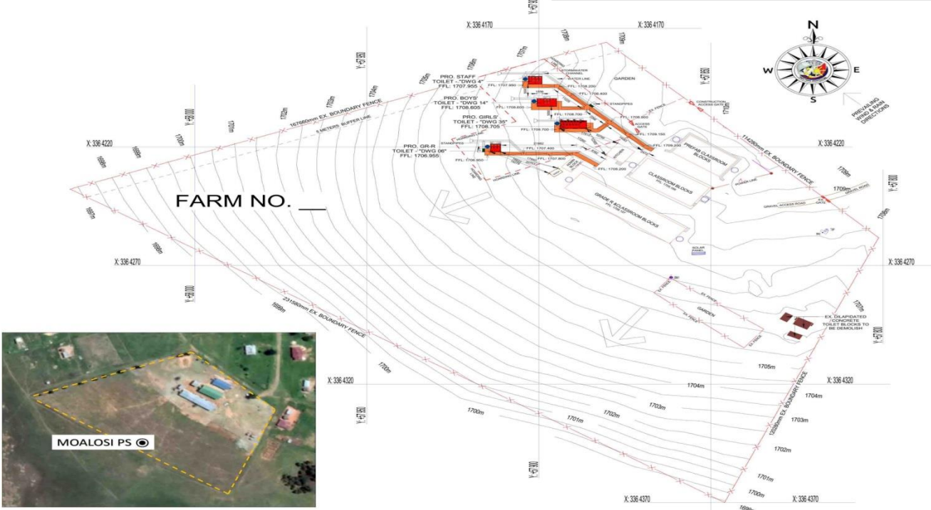
1 SITE DEVELOPMENT PLAN - REV00 1 : 500
