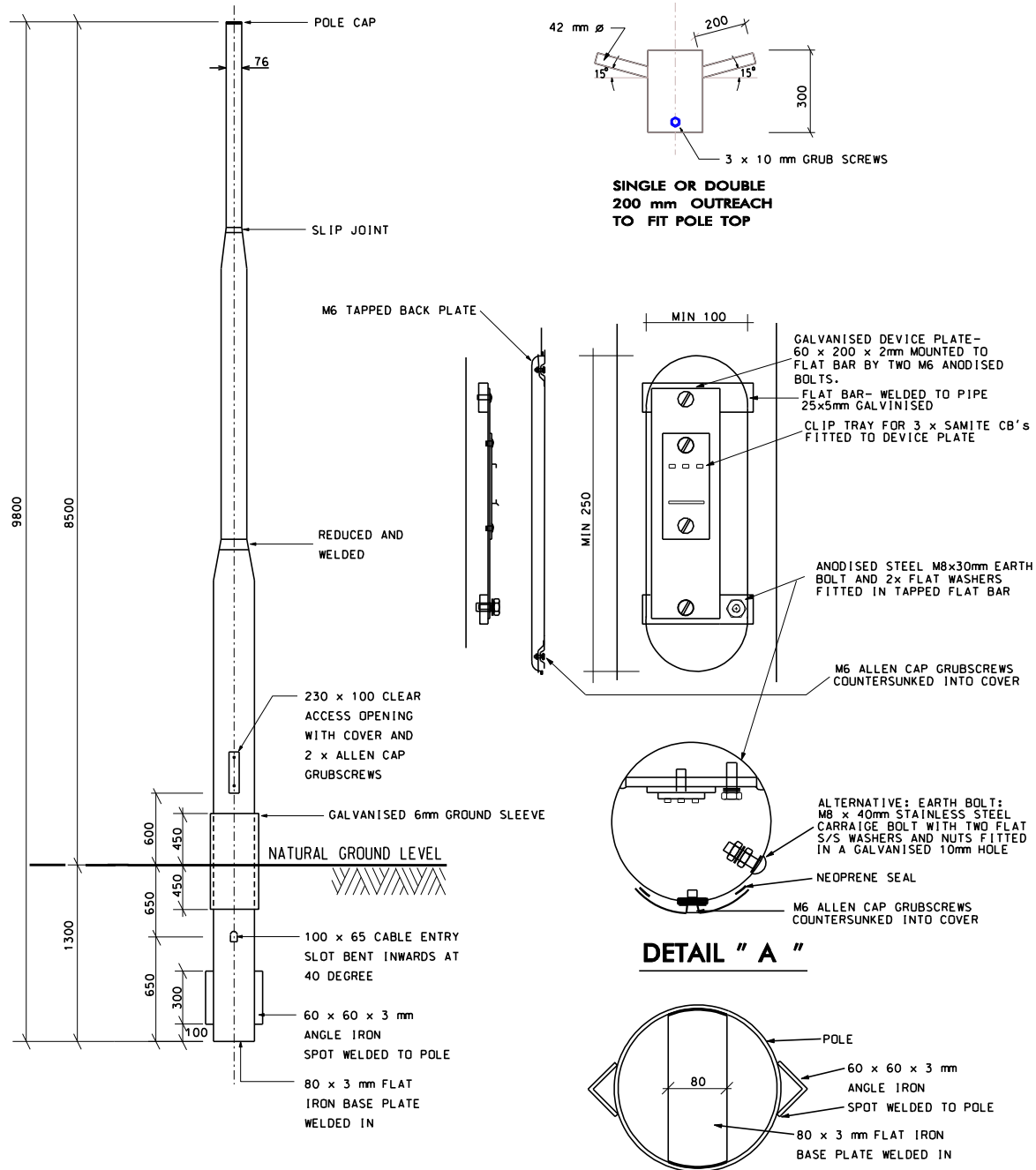
BASE PLATE DETAIL
