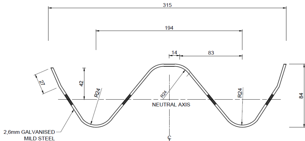
SECTION THROUGH GUARDRAIL
