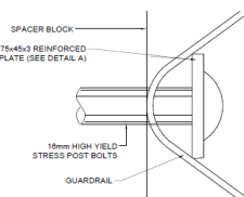
REINFORCING PLATE DETAIL DETAIL OF BULLNOSE
