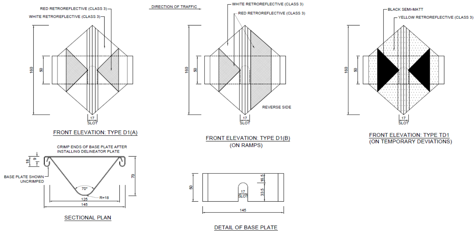
DETAIL OF GUARDRAIL DELINEATORS
