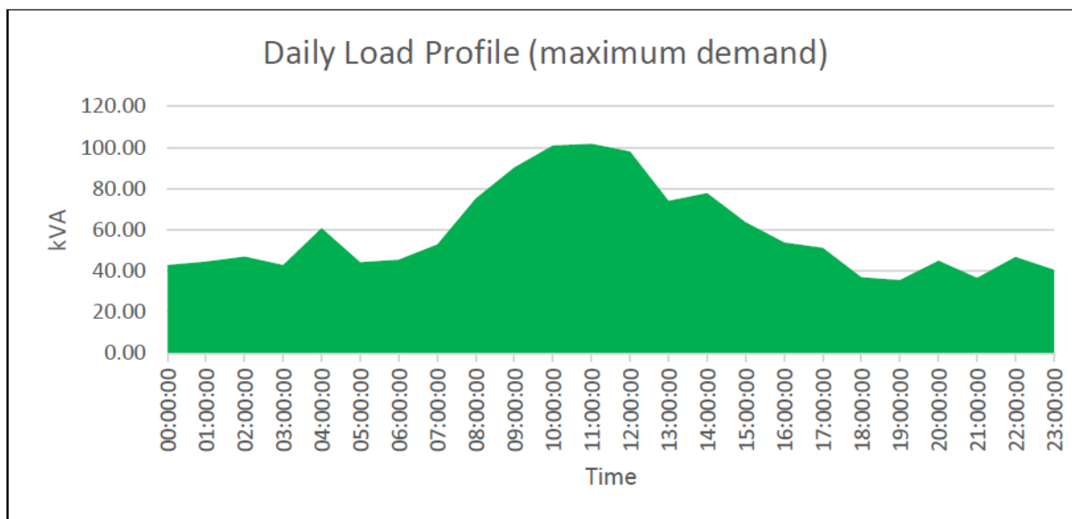
Figure 7: Maximum Demand for 12 th June
