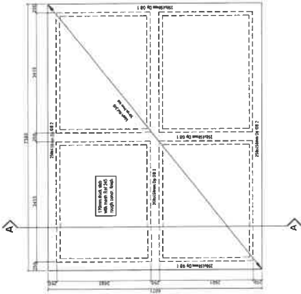
W1A-R: RAFT FOUNDATION AND PIT SLAB LAYOUT PLAN
