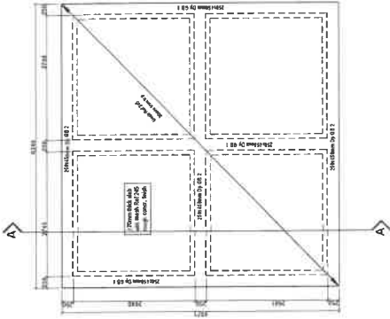
W1A-T: RAFT FOUNDATION AND PIT SLAB LAYOUT PLAN
