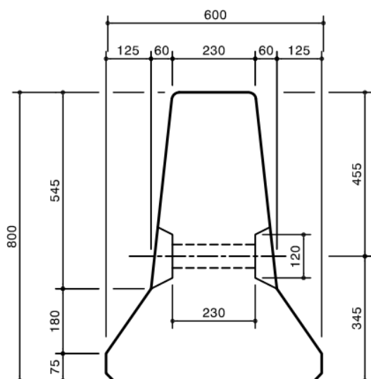
Figure 1: cross section – new Jersey Barrier
