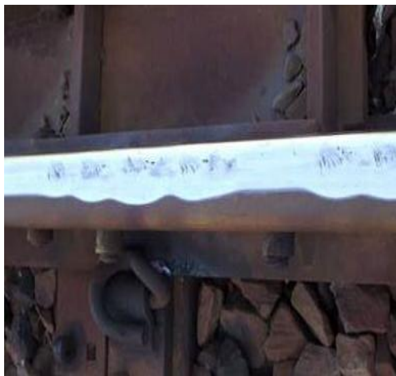
Figure 2: Wheel spin burns (skid marks)
