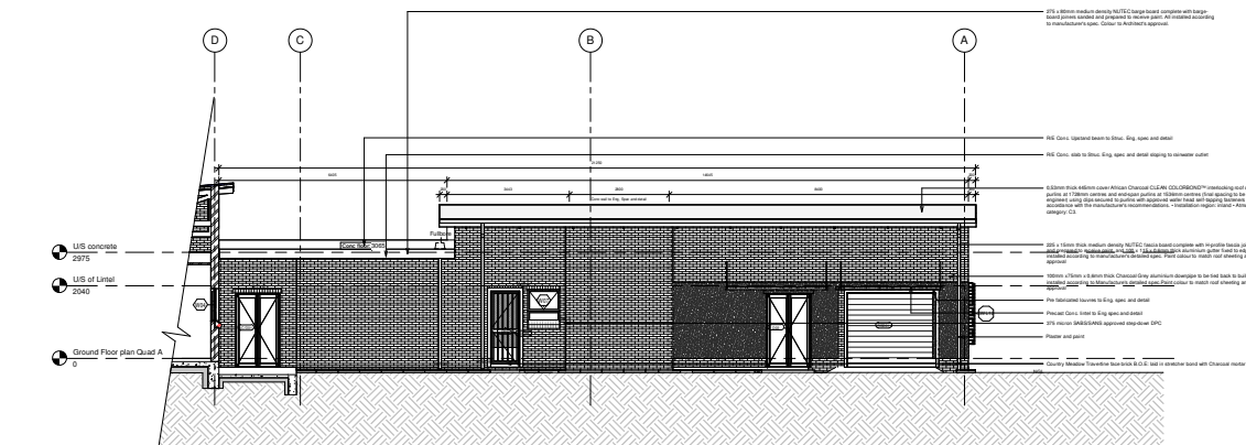
1 North Eastern sectional elevation 1:50
