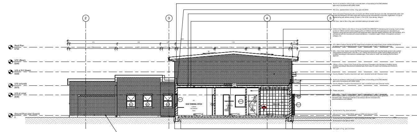
2 North Western sectional elevation 1:50
