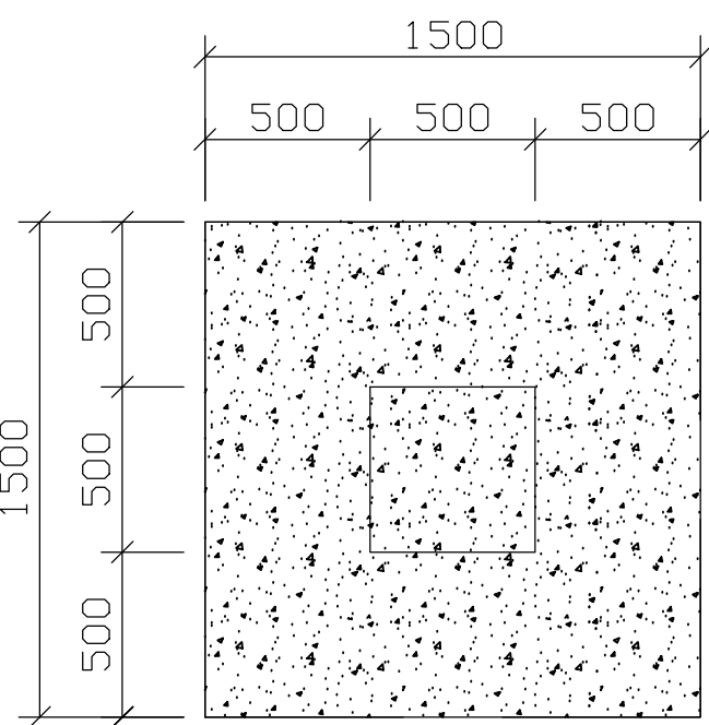
FOUNDATION LAYOUT
