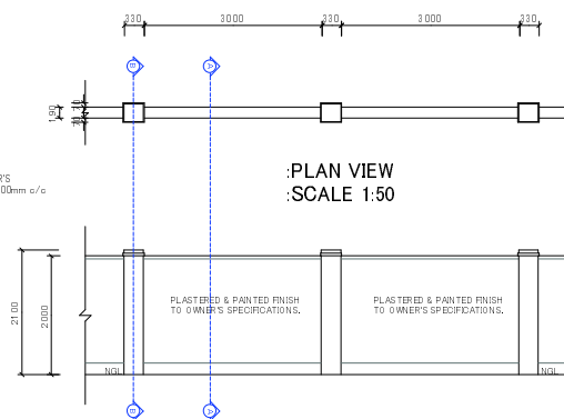
:ELEVATION VIEW :SCALE 1:50
