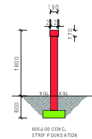
:SCREED WALL DETAIL :SCALE 1:50
