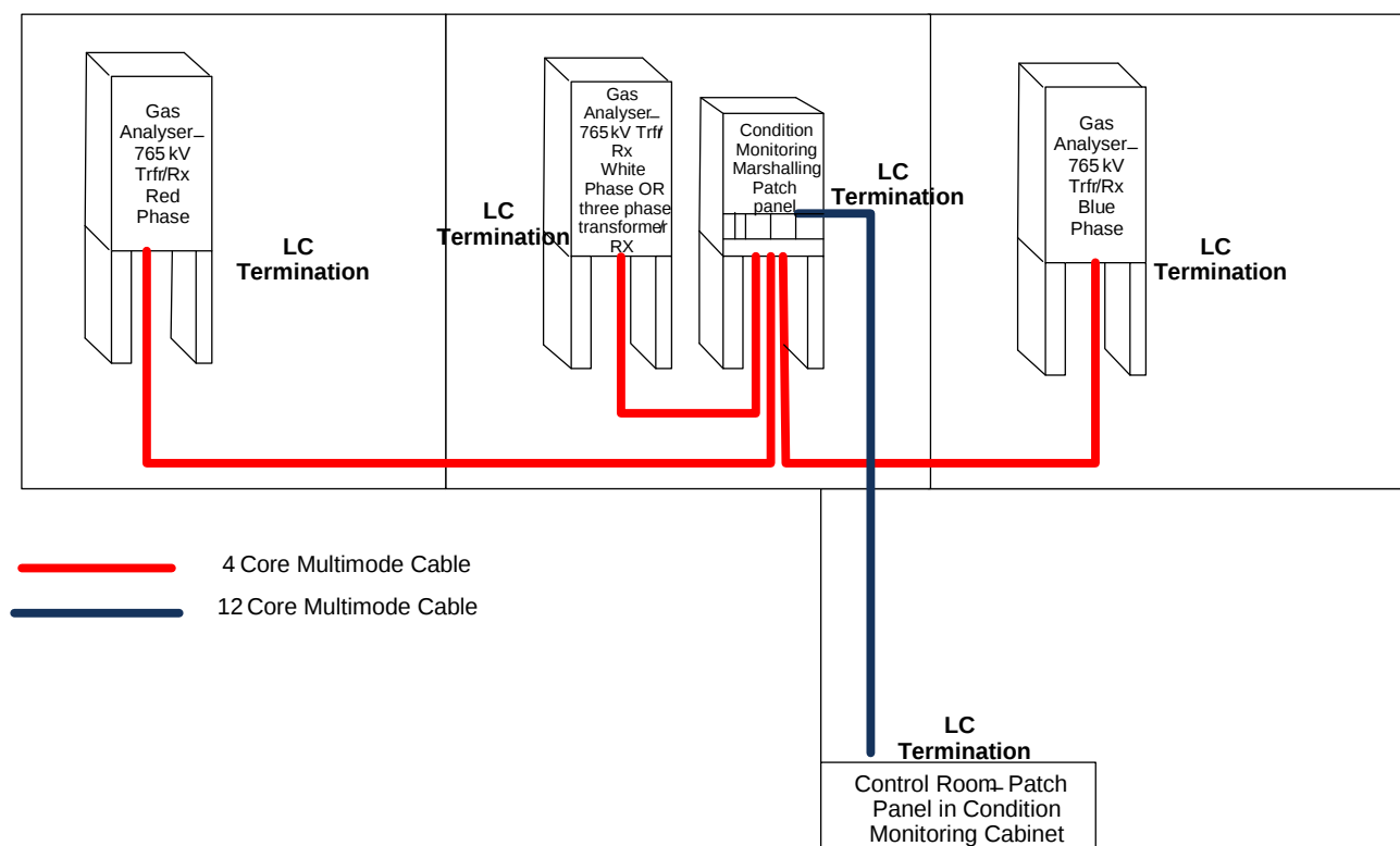
Figure 3: Typical layout and cabling of analyser, transformer patch panel and control room patch panel for three single phase transformers. This layout would also be used when power transformers are within 10 metres to one-another.
