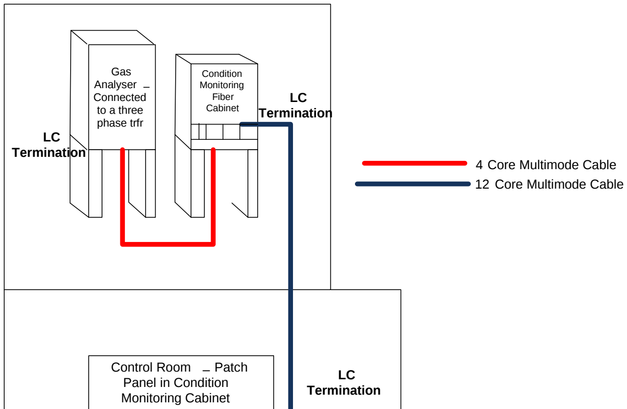
Figure 2: Typical layout and cabling of analyser, transformer patch panel and control room patch panel for a three-phase transformer.
