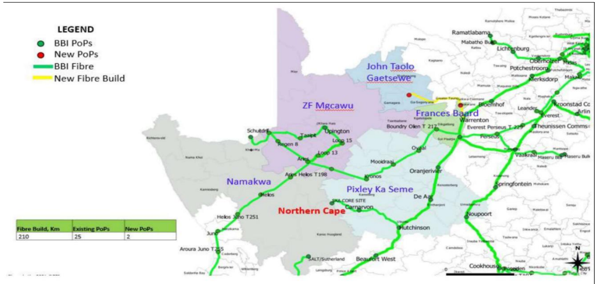
Figure 1: Northern Cape province fibre footprint and planned PoP sites.
