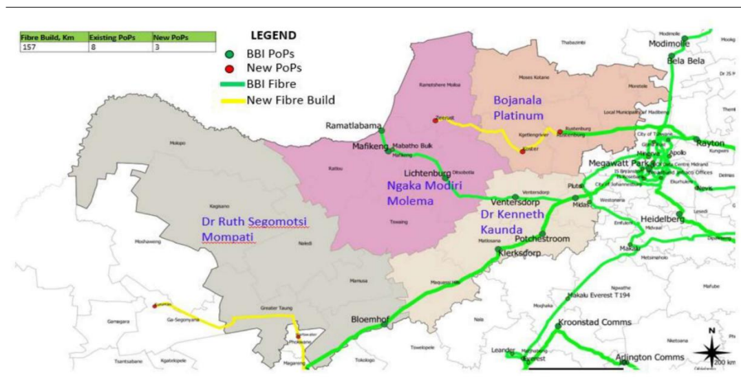
Figure 1: North-West province fibre footprint and planned PoP sites.
