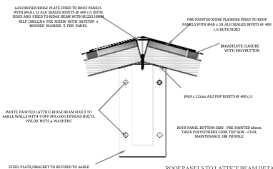
ROOF PANELS TO LATTICE BEAM DETAIL
