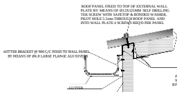
ROOF TO GUTTER DETAIL
