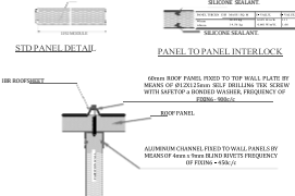
INTERNAL PARTITION WALL TO ROOF FIXING DETAIL
