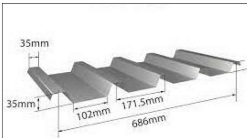
Profile of 0.5mm IBR roof sheet
