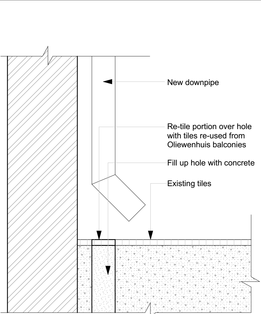
Detail 100-02 - DOWNPIPE DETAIL Scale 1:10
