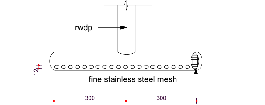
Detail 100-04 - SPREADER DETAIL Scale 1:10
