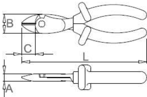
Figure 16: Side Cutter Drawing
