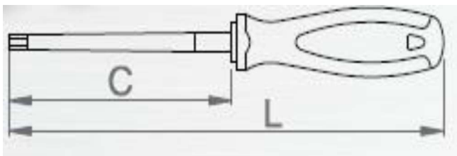
Figure 7: Hexagon Screwdriver
