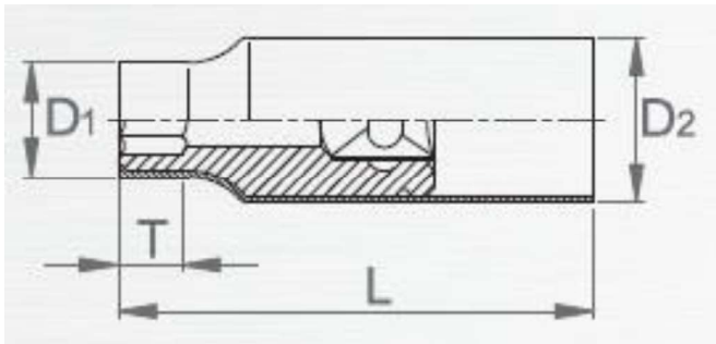
Figure 18: Socket Drawing
