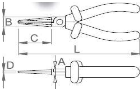
Figure 9: Longnose Pliers Drawing
