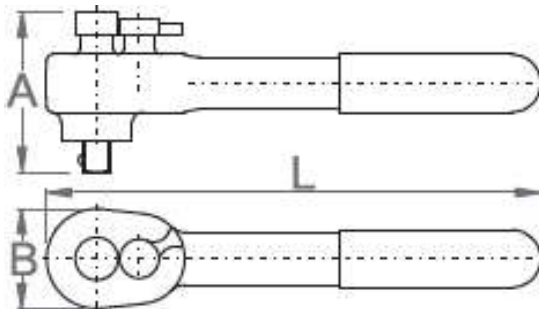
Figure 13: Reversible ratchet Drawing
