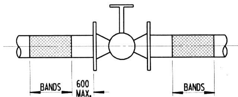
Figure D.7.1 — Colour identification around in-line equipment
