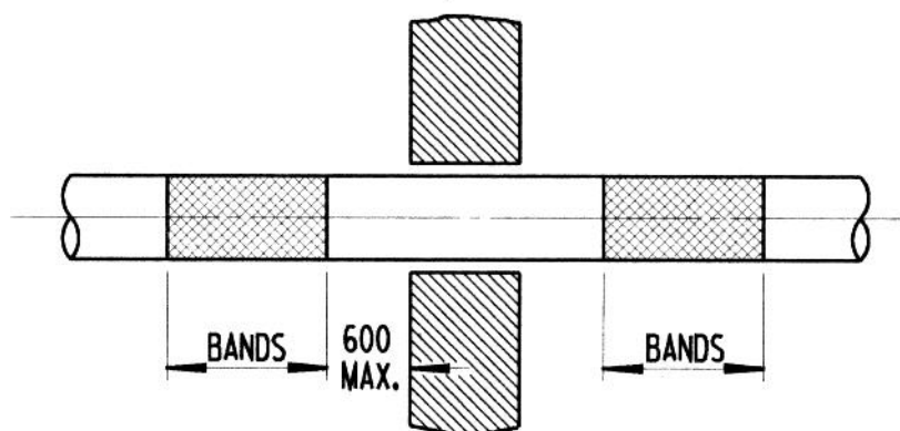
Figure D.7.2 — Colour identification at bulkheads, wall penetrations and floors
