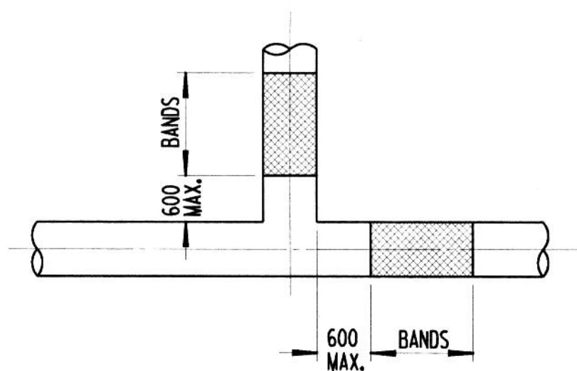
Figure D.7.3 — Colour identification at piping junctions or connections
