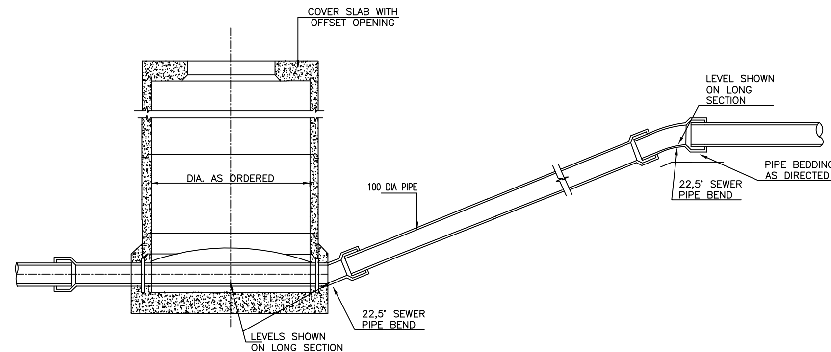
MANHOLE CHAMBER WITH 22.5 DEG RAMP
