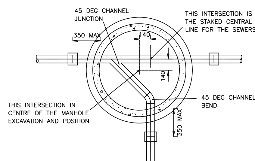
90 DEG JUNCTION TYPE 8
