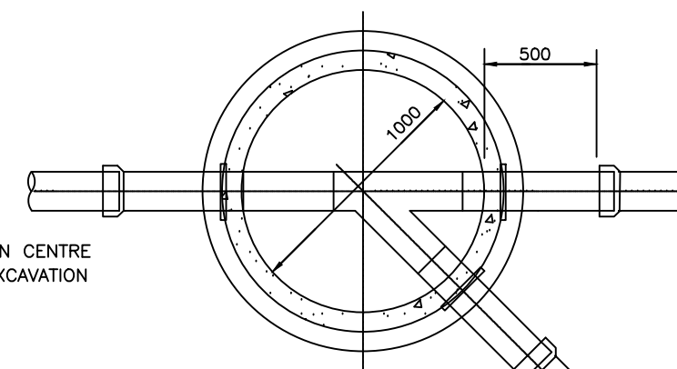
45 DEG JUNCTION TYPE 5
