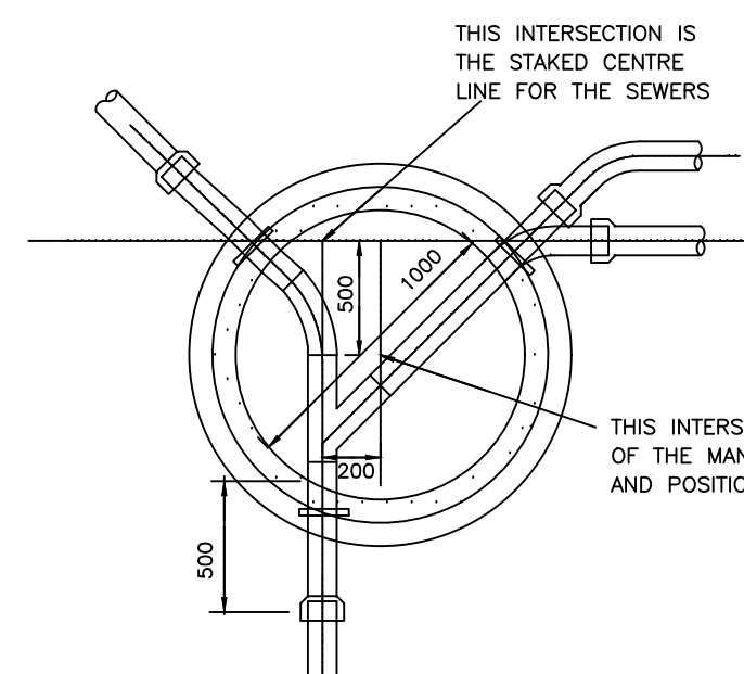
TEE JUNCTION TYPE 4
