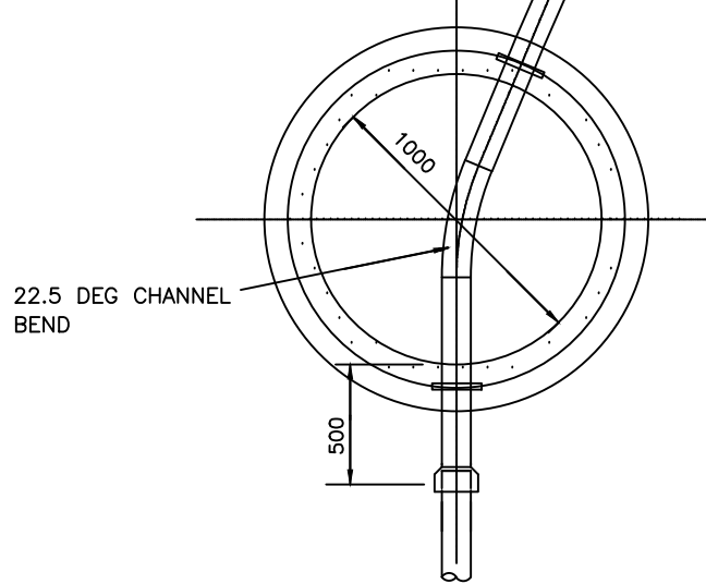
22.5 DEG BEND TYPE 7a
