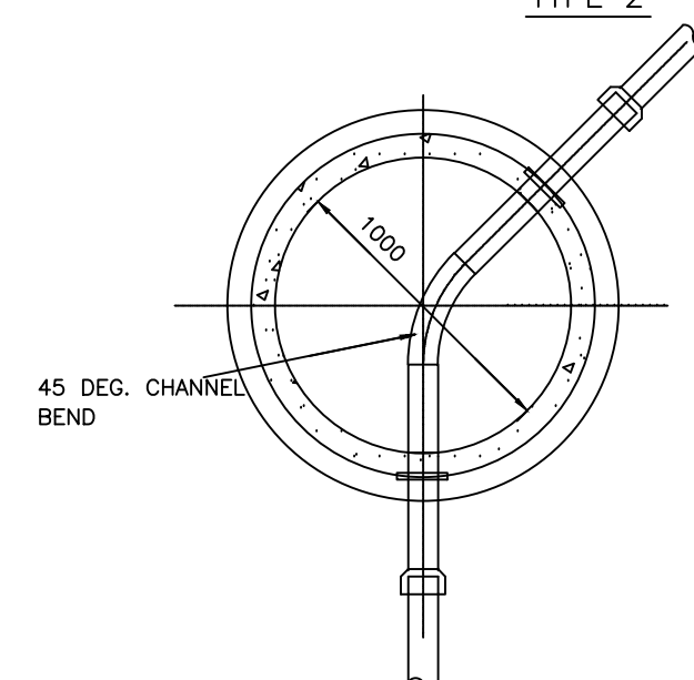
45 DEG BEND TYPE 7b
