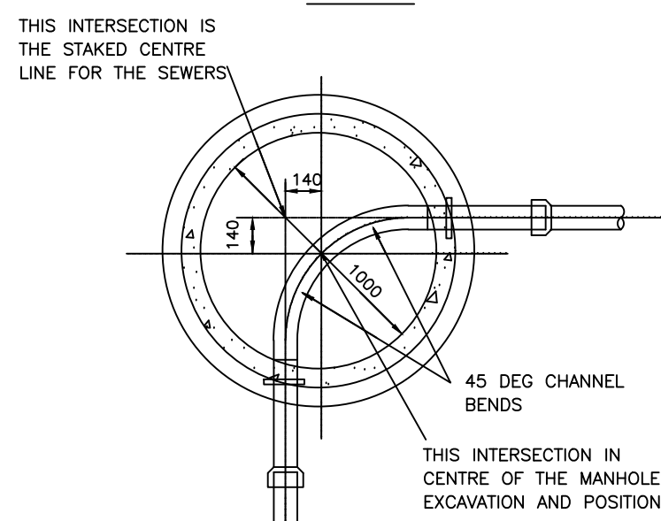
TEE JUNCTION TYPE 4
