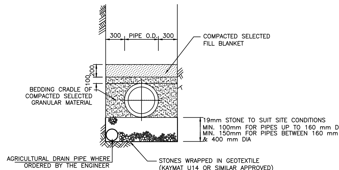
TYPICAL TRENCH SECTION IN WATERLOGGED AREAS
