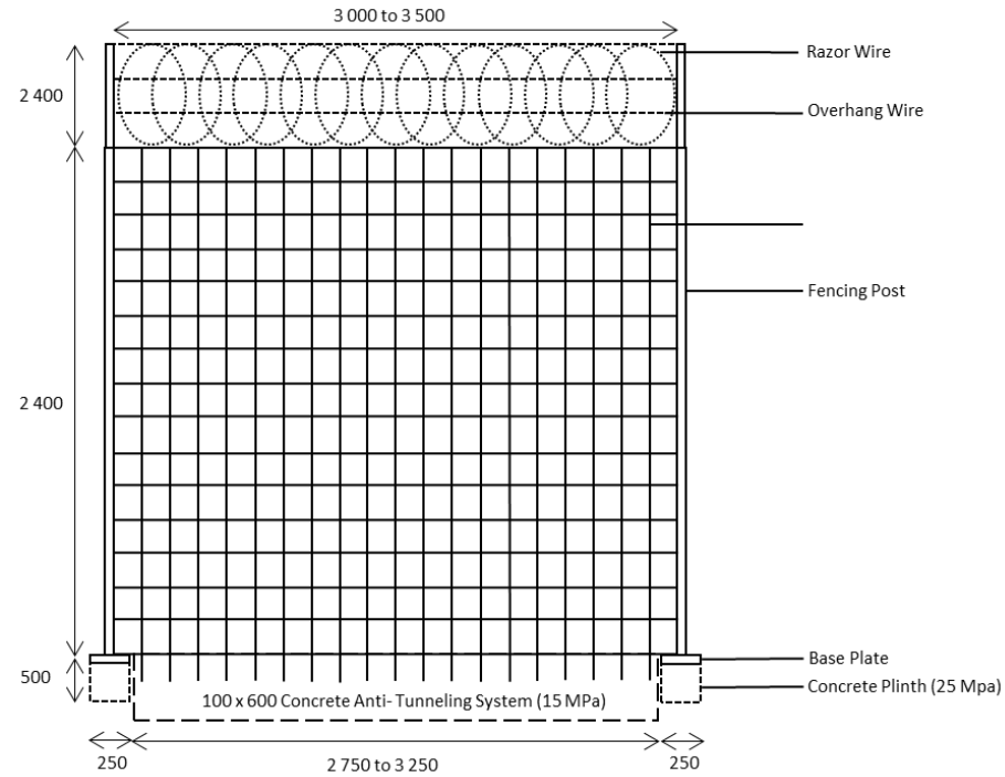
Figure 2: Cross Section of Fencing Layout
