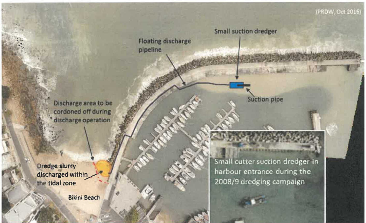
Figure 1: Indicative maintenance dredging operation and dredge material discharge.
