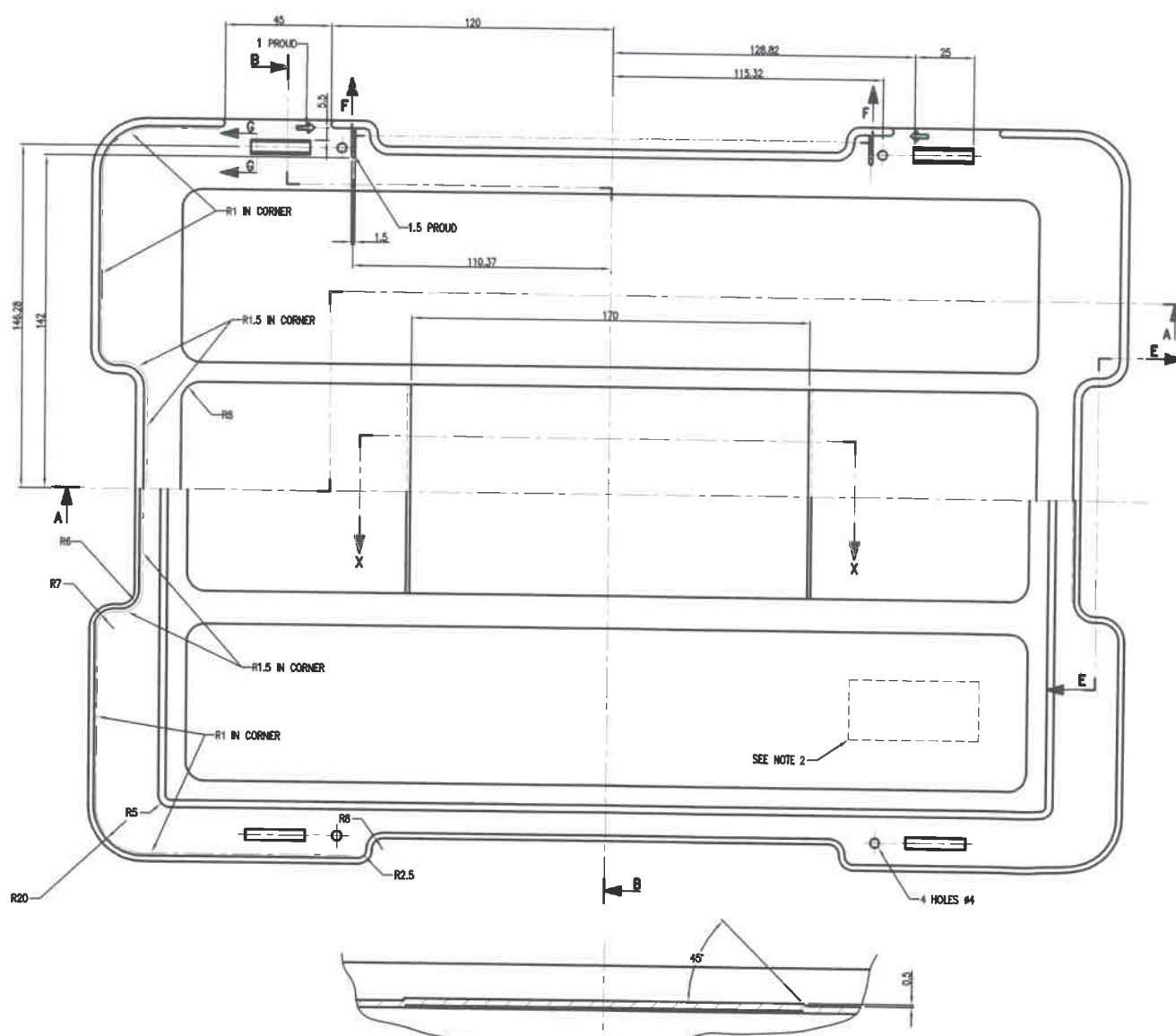
SCRAP SECTION X-X
