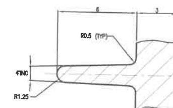
ENLARGED DETAIL Z
