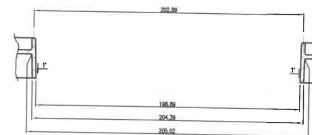
SECTION F-F
