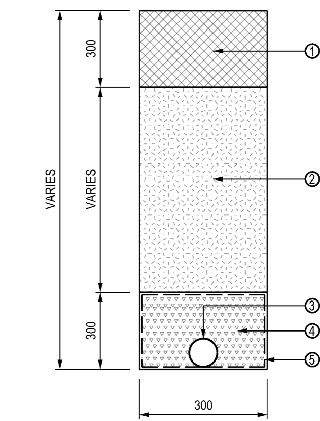
TYPICAL SECTION THROUGH SUBSOIL DRAIN SCALE 1:15
