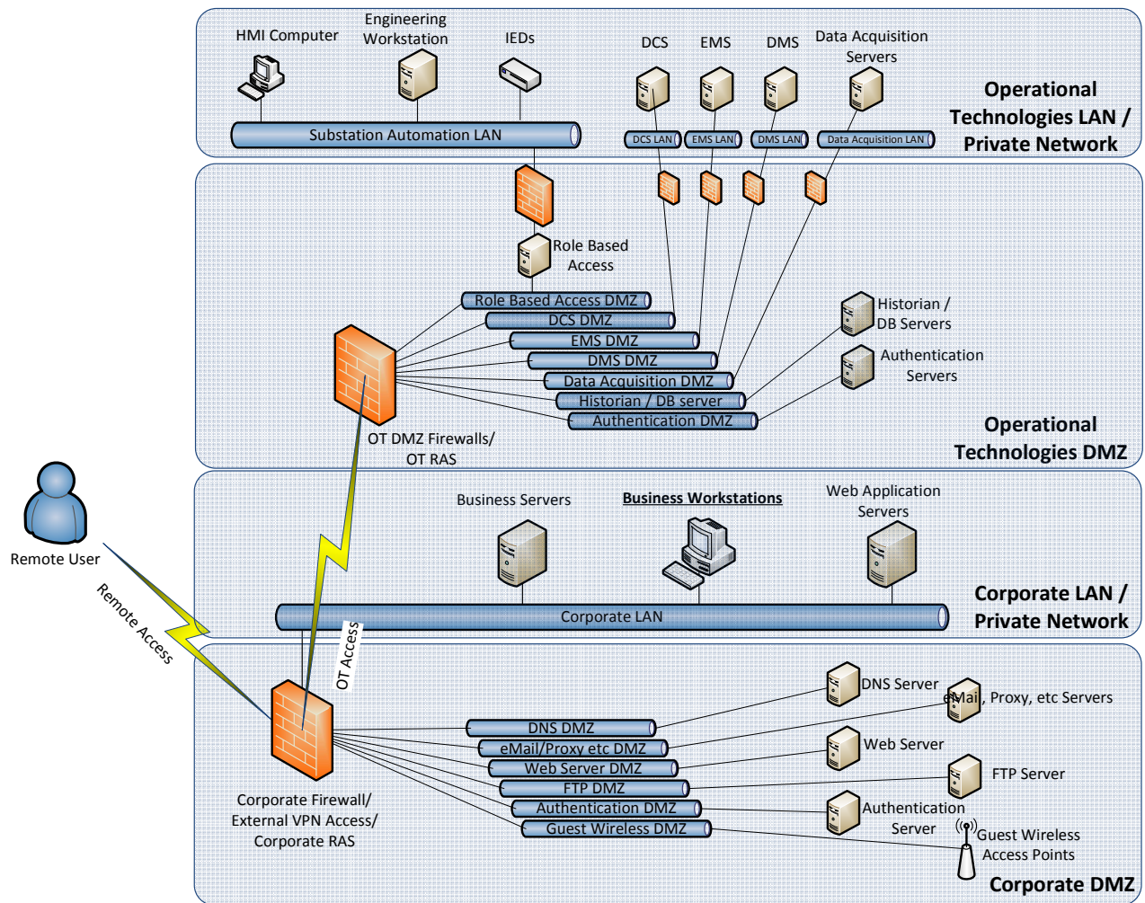
Figure 1: Remote Access Architecture
