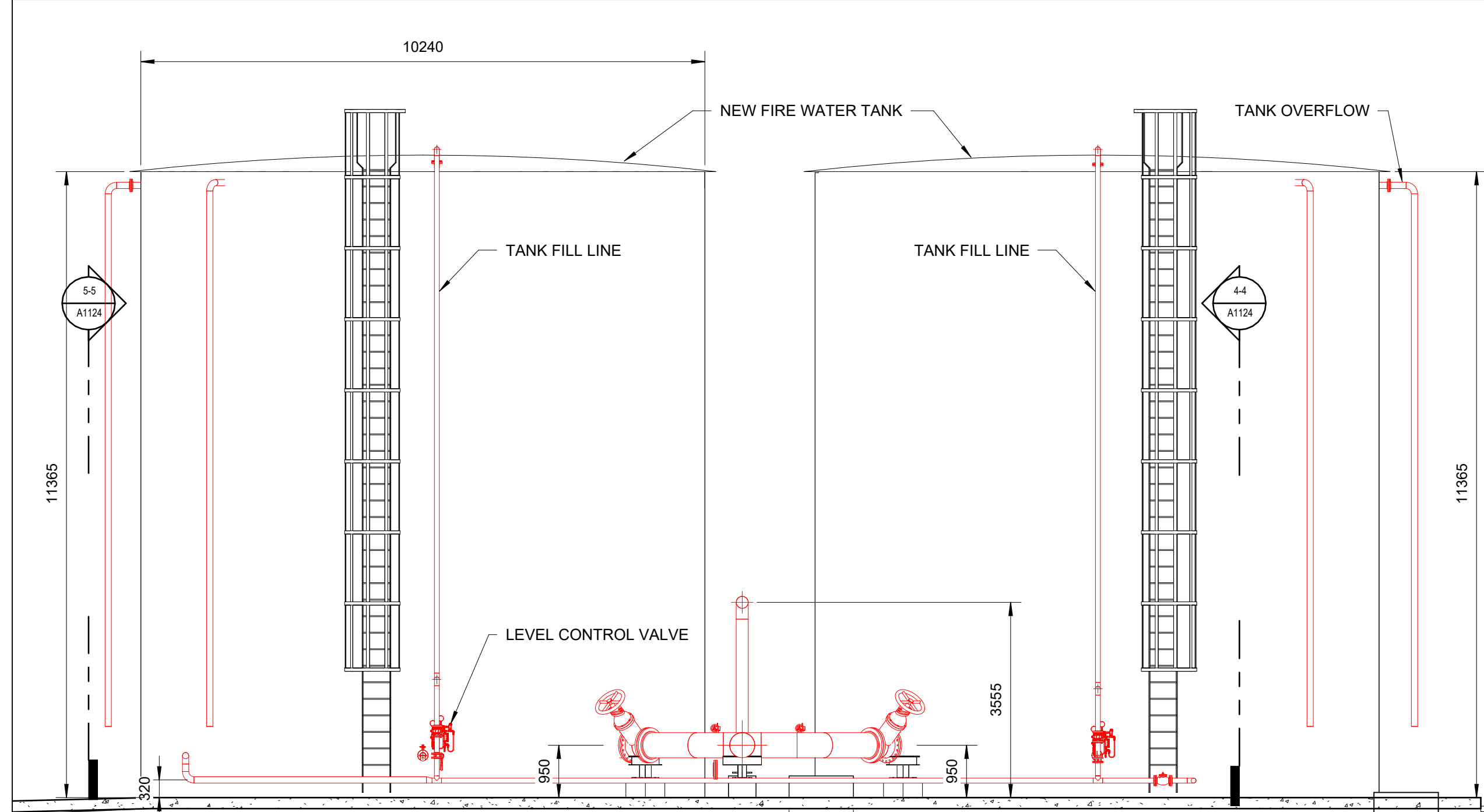
SECTION 1-1 : WATER TANKS
