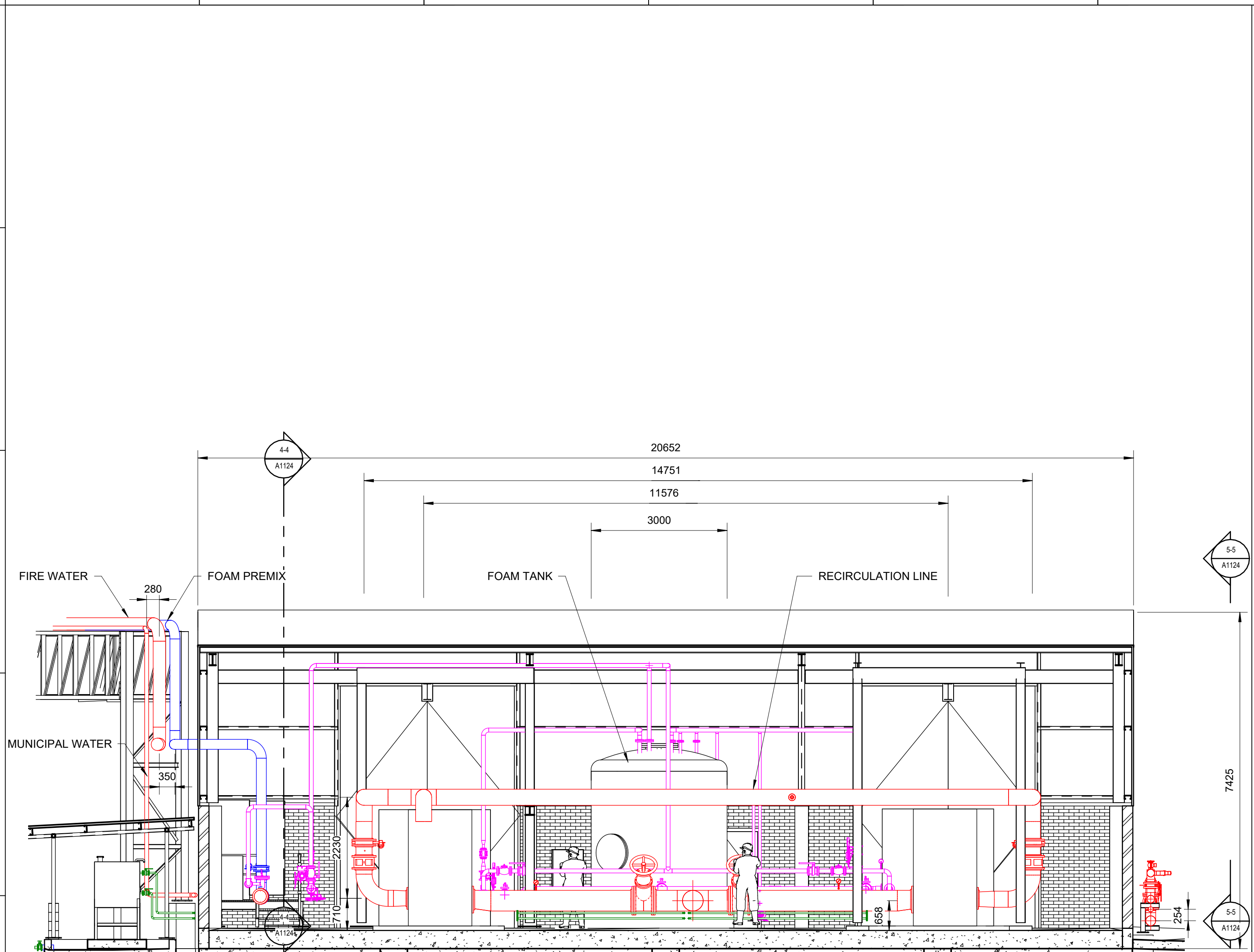
SECTION 2-2 : PUMP HOUSE BACK VIEW
