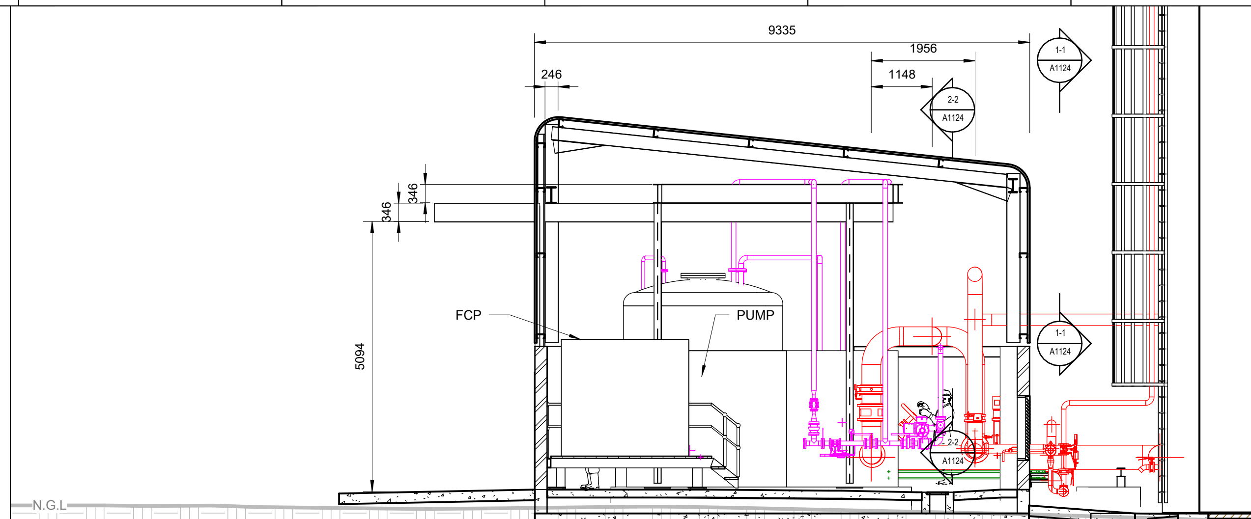
SECTION 4-4 : PUMP HOUSE RIGHT VIEW
