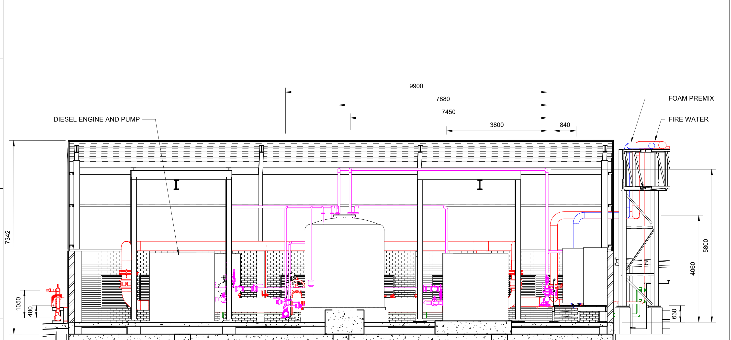
SECTION 3-3 : PUMP HOUSE FRONT VIEW
