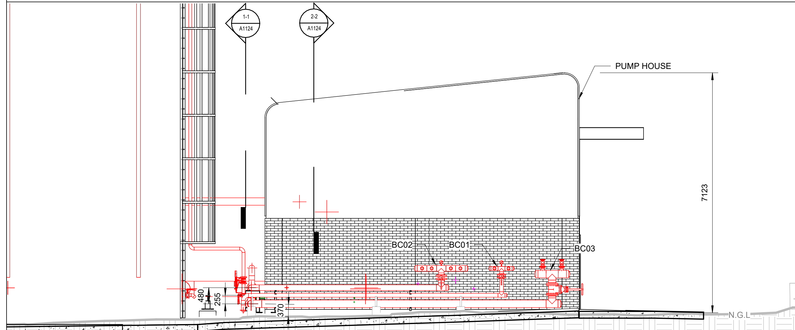
SECTION 5-5 : PUMP HOUSE LEFT VIEW
