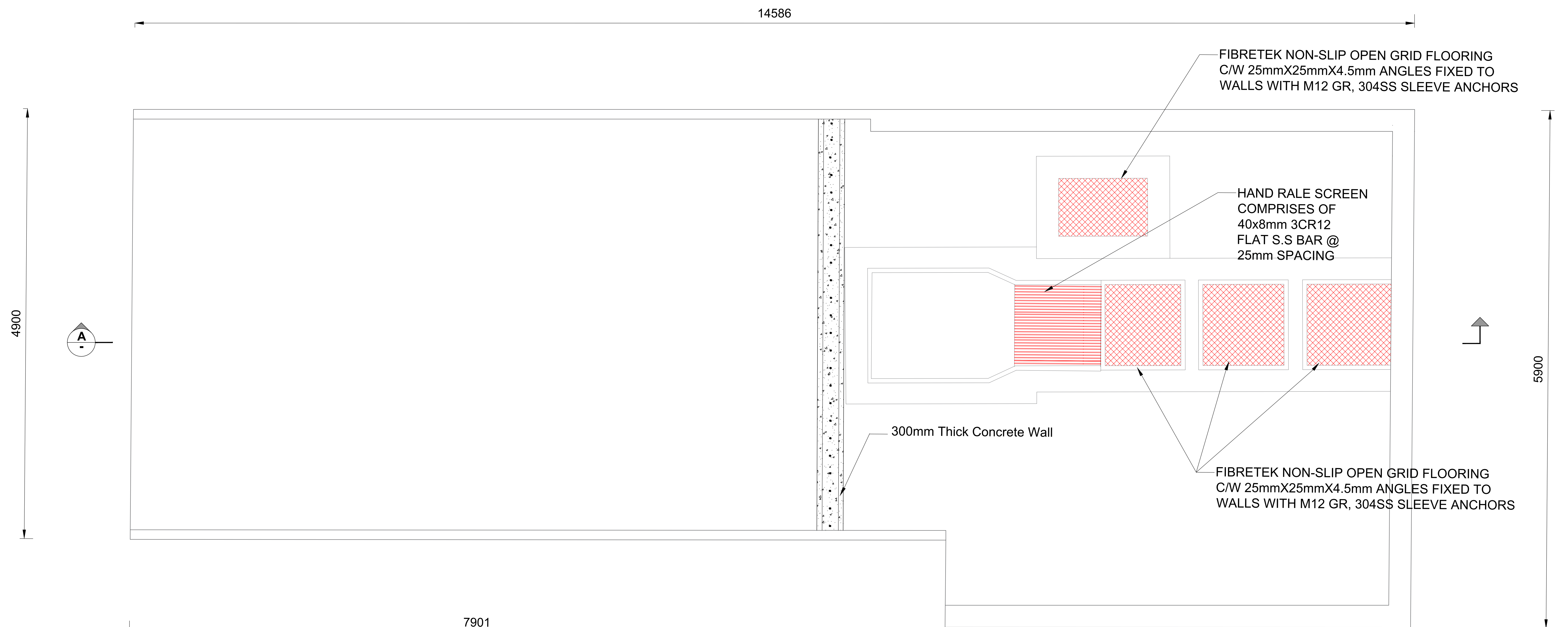
PLAN LAYOUT
