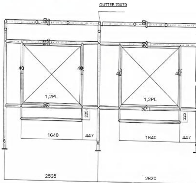
FRONT ELEV
