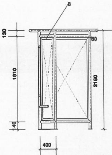
LEFT VIEW
