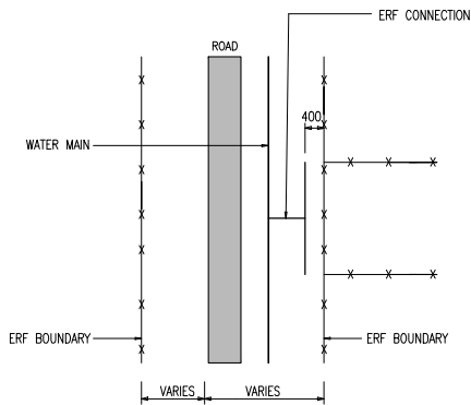
PLAN: TYPE 9
