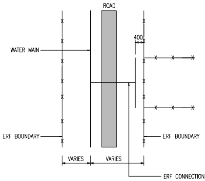
PLAN: TYPE 10
