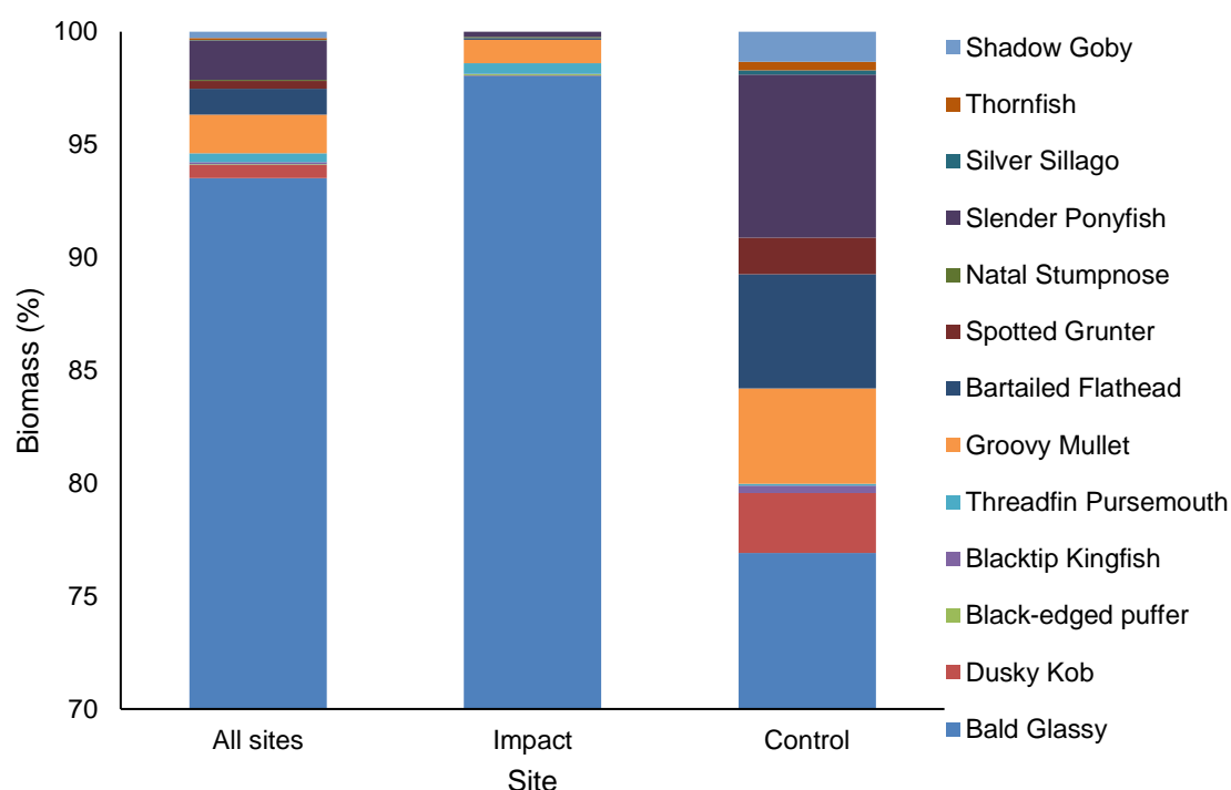
Figure 16: Relative mass (%) of fish species caught overall (all sites) and at impact and control sites. Note that the y-axis starts at 70%.
