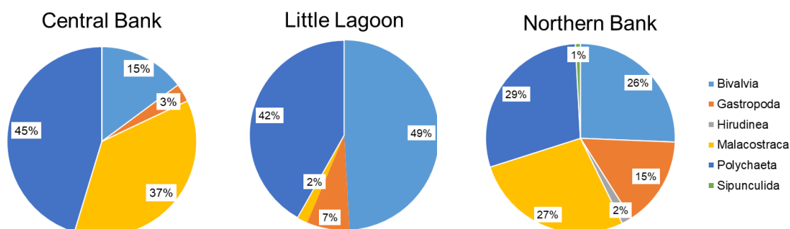
Figure 8: Percentage abundance of subtidal macrofauna classes in communities of the central bank, little lagoon and northern bank.
