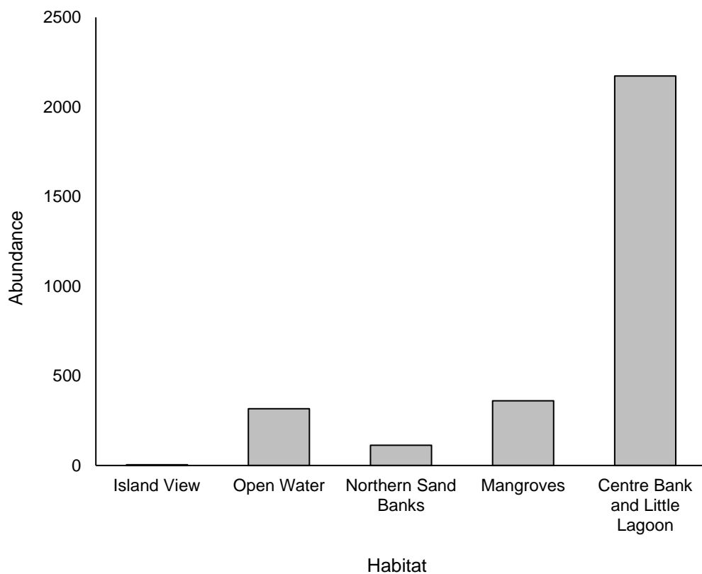
Figure 21: Total bird abundance per habitat recorded during monthly counts from March – May 2021.
