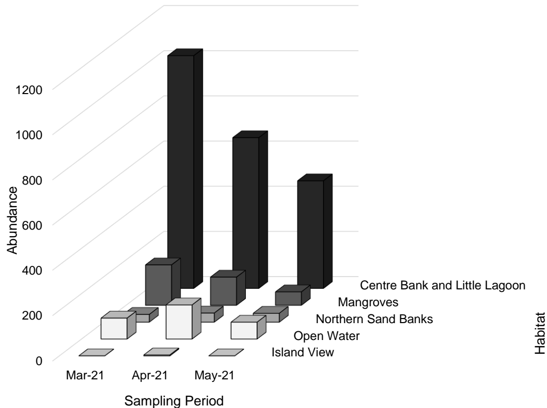
Figure 22: Monthly bird abundance per habitat recorded from March – May 2021.
