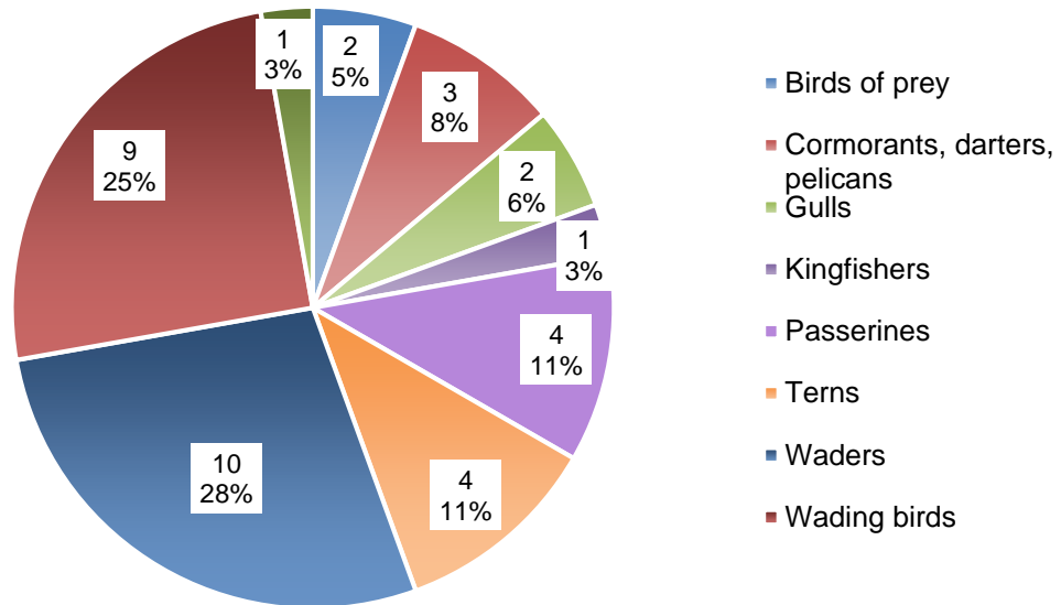
Figure 19: Taxonomic composition (number and percentage of species) of bird communities recorded during monthly counts from March - May 2021.
