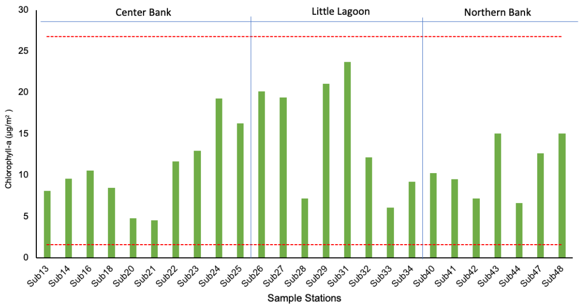
Figure 11: Chlorophyll-a concentrations ( \mu\text{g}/\text{m}^2 ) in 25 subtidal monitoring stations in the Port of Durban, autumn 2021. Impact sites = Sub13 – Sub34, control sites = Sub40 – Sub48. Red dotted lines: 20%tile ( 1.6 \mu\text{g}/\text{m}^2 ) and 80%tile ( 26.8 \mu\text{g}/\text{m}^2 ) subtidal autumn threshold limits stipulated in the CSMP.
