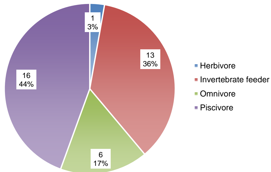
Figure 20: Composition of feeding guilds (number and percentage of species) recorded during monthly counts from March - May 2021.
