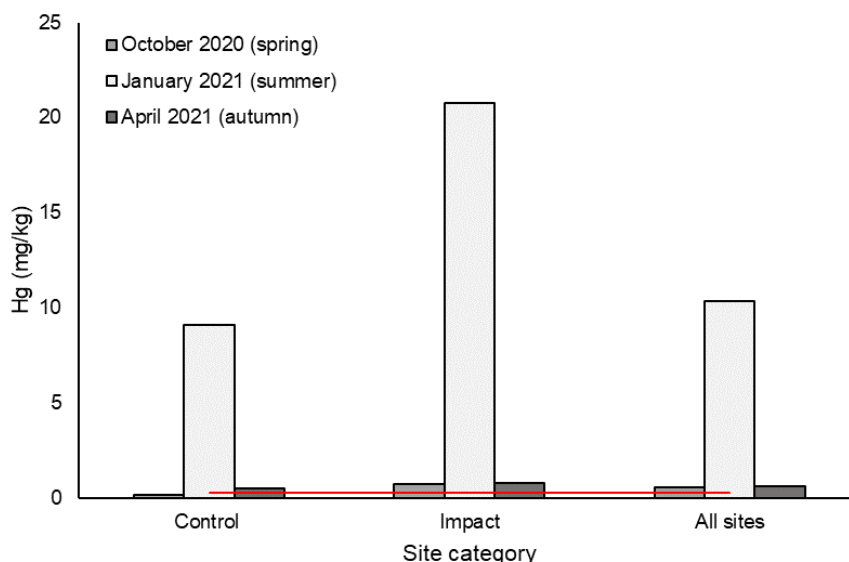
Figure 13: Median mercury concentrations (mg/kg) quantified from October 2020 (spring) to April 2021 (autumn). Red line = baseline threshold value (0.29306 mg/kg).
