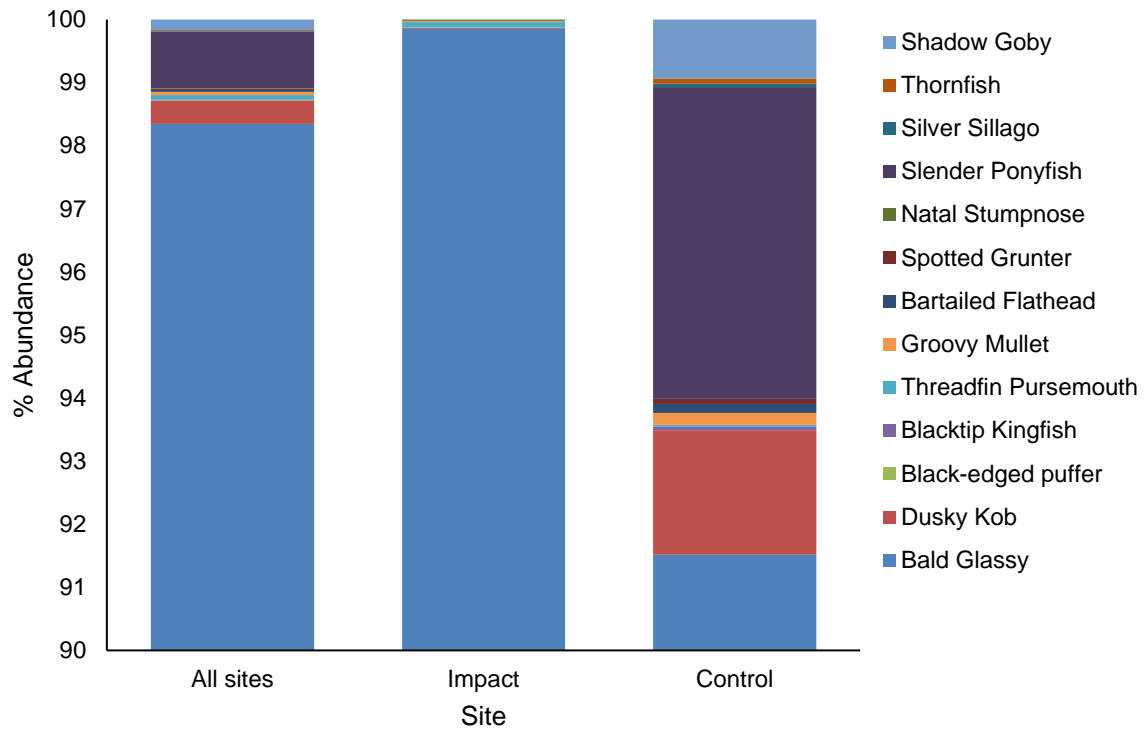
Figure 15: Relative abundance (%) of fish species caught overall (all sites) and at impact and control sites. Note that the y-axis starts at 90%.
